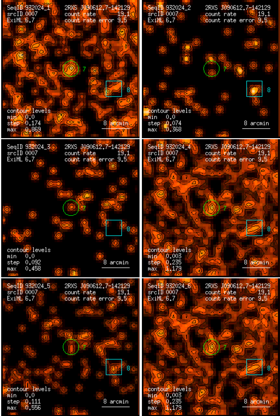
Figure 7: RASS 932024: detection 0007: band rate images, Gaussian filter: (1) PSPC channels 11 – 41, (2) 52 – 90, (3) 91 – 201, (4) 11 – 235, (5) 52 – 201, (6) 11 – 201. Broad band rates in counts/ks. Band rate contour levels in counts/ks/arcmin 2 .
