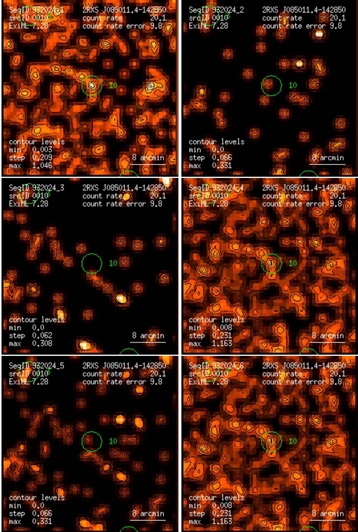
Figure 10: RASS 932024: detection 0010: band rate images, Gaussian filter: (1) PSPC channels 11 – 41, (2) 52 – 90, (3) 91 – 201, (4) 11 – 235, (5) 52 – 201, (6) 11 – 201. Broad band rates in counts/ks. Band rate contour levels in counts/ks/arcmin 2 .
