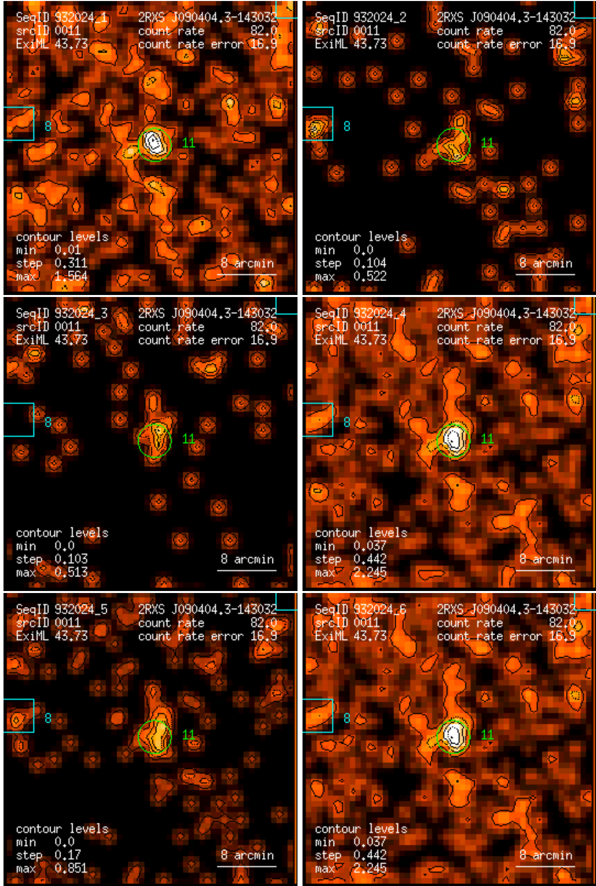
Figure 11: RASS 932024: detection 0011: band rate images, Gaussian filter: (1) PSPC channels 11 – 41, (2) 52 – 90, (3) 91 – 201, (4) 11 – 235, (5) 52 – 201, (6) 11 – 201. Broad band rates in counts/ks. Band rate contour levels in counts/ks/arcmin 2 .
