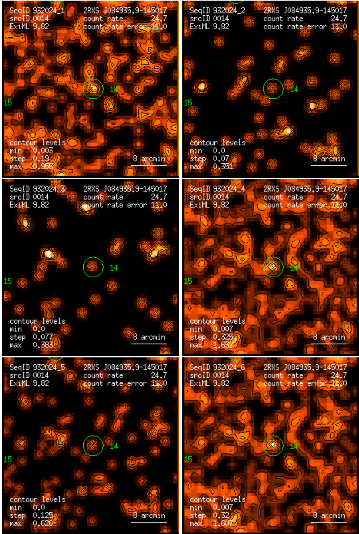
Figure 14: RASS 932024: detection 0014: band rate images, Gaussian filter: (1) PSPC channels 11 – 41, (2) 52 – 90, (3) 91 – 201, (4) 11 – 235, (5) 52 – 201, (6) 11 – 201. Broad band rates in counts/ks. Band rate contour levels in counts/ks/arcmin 2 .
