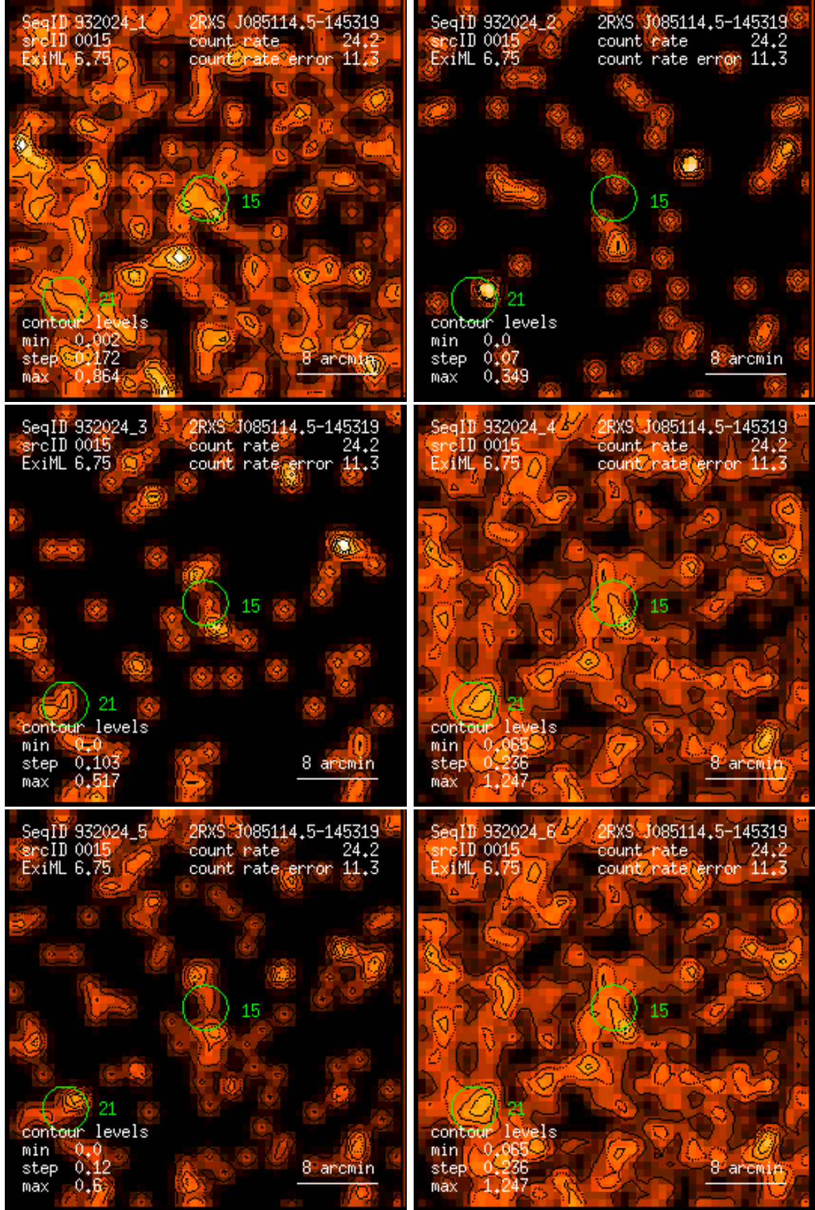
Figure 15: RASS 932024: detection 0015: band rate images, Gaussian filter: (1) PSPC channels 11 – 41, (2) 52 – 90, (3) 91 – 201, (4) 11 – 235, (5) 52 – 201, (6) 11 – 201. Broad band rates in counts/ks. Band rate contour levels in counts/ks/arcmin 2 .
