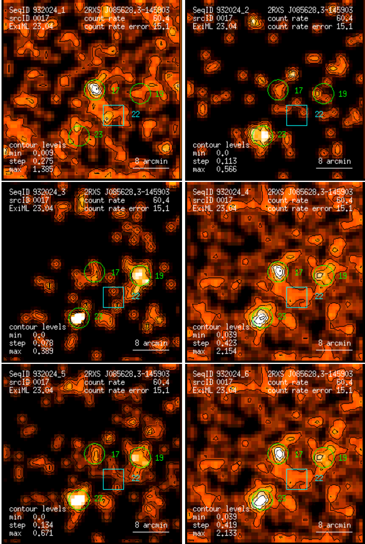
Figure 17: RASS 932024: detection 0017: band rate images, Gaussian filter: (1) PSPC channels 11 – 41, (2) 52 – 90, (3) 91 – 201, (4) 11 – 235, (5) 52 – 201, (6) 11 – 201. Broad band rates in counts/ks. Band rate contour levels in counts/ks/arcmin 2 .
