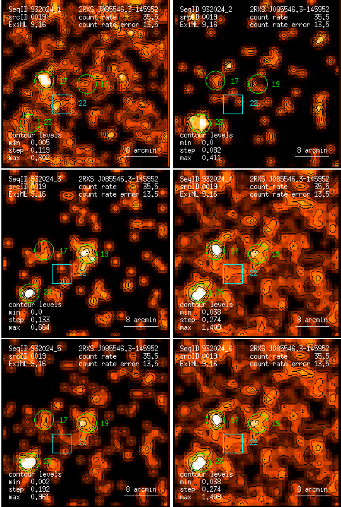
Figure 19: RASS 932024: detection 0019: band rate images, Gaussian filter: (1) PSPC channels 11 – 41, (2) 52 – 90, (3) 91 – 201, (4) 11 – 235, (5) 52 – 201, (6) 11 – 201. Broad band rates in counts/ks. Band rate contour levels in counts/ks/arcmin 2 .
