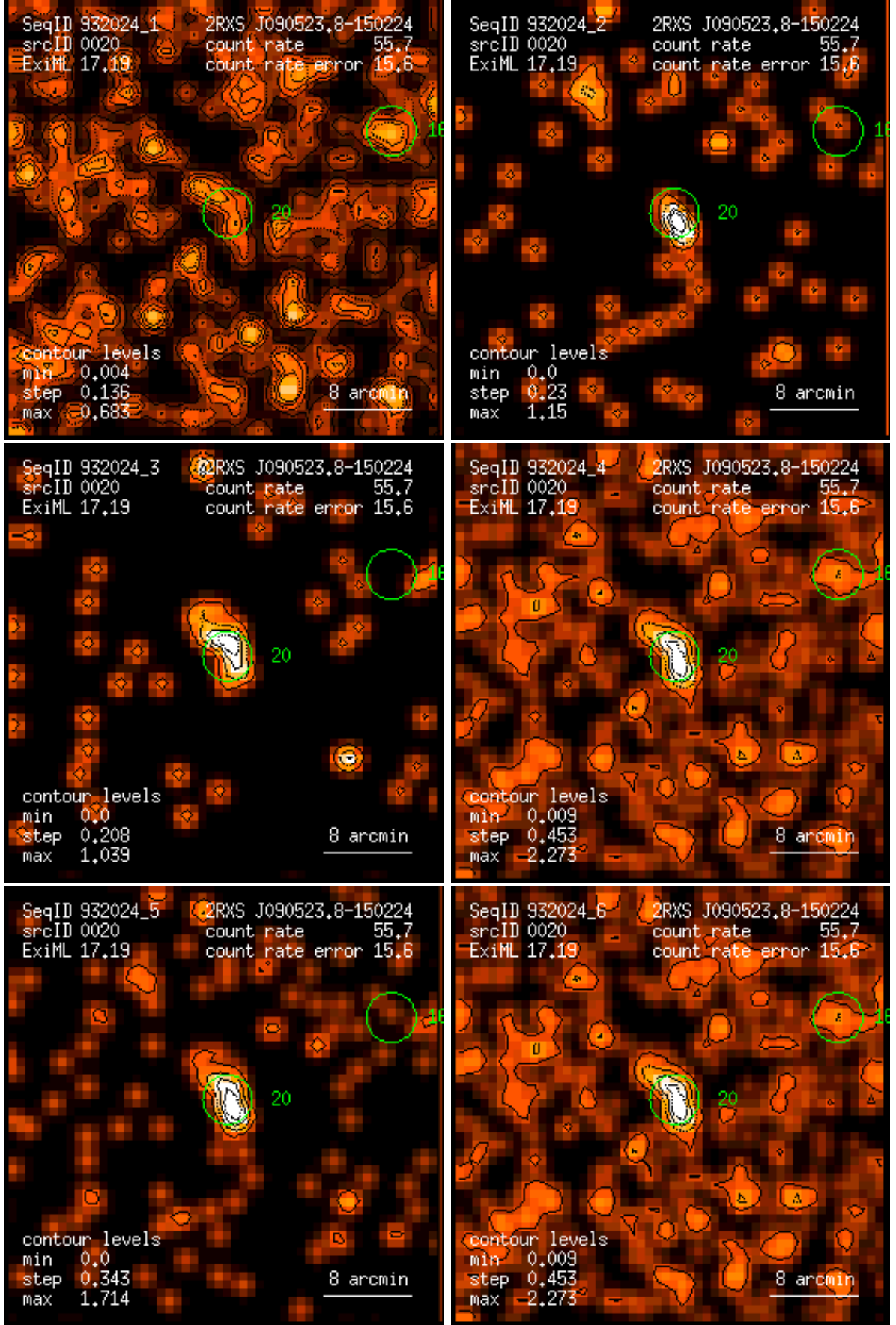
Figure 20: RASS 932024: detection 0020: band rate images, Gaussian filter: (1) PSPC channels 11 – 41, (2) 52 – 90, (3) 91 – 201, (4) 11 – 235, (5) 52 – 201, (6) 11 – 201. Broad band rates in counts/ks. Band rate contour levels in counts/ks/arcmin 2 .
