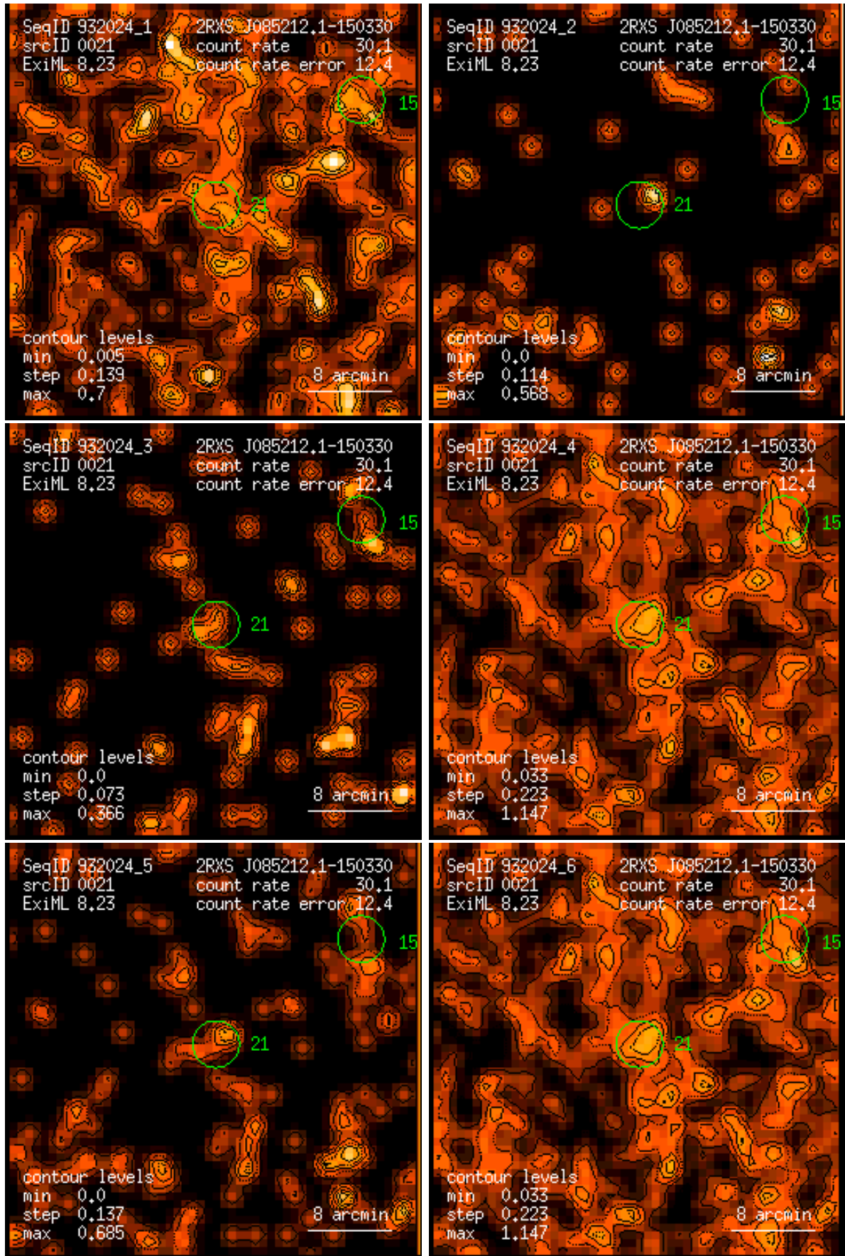
Figure 21: RASS 932024: detection 0021: band rate images, Gaussian filter: (1) PSPC channels 11 – 41, (2) 52 – 90, (3) 91 – 201, (4) 11 – 235, (5) 52 – 201, (6) 11 – 201. Broad band rates in counts/ks. Band rate contour levels in counts/ks/arcmin 2 .
