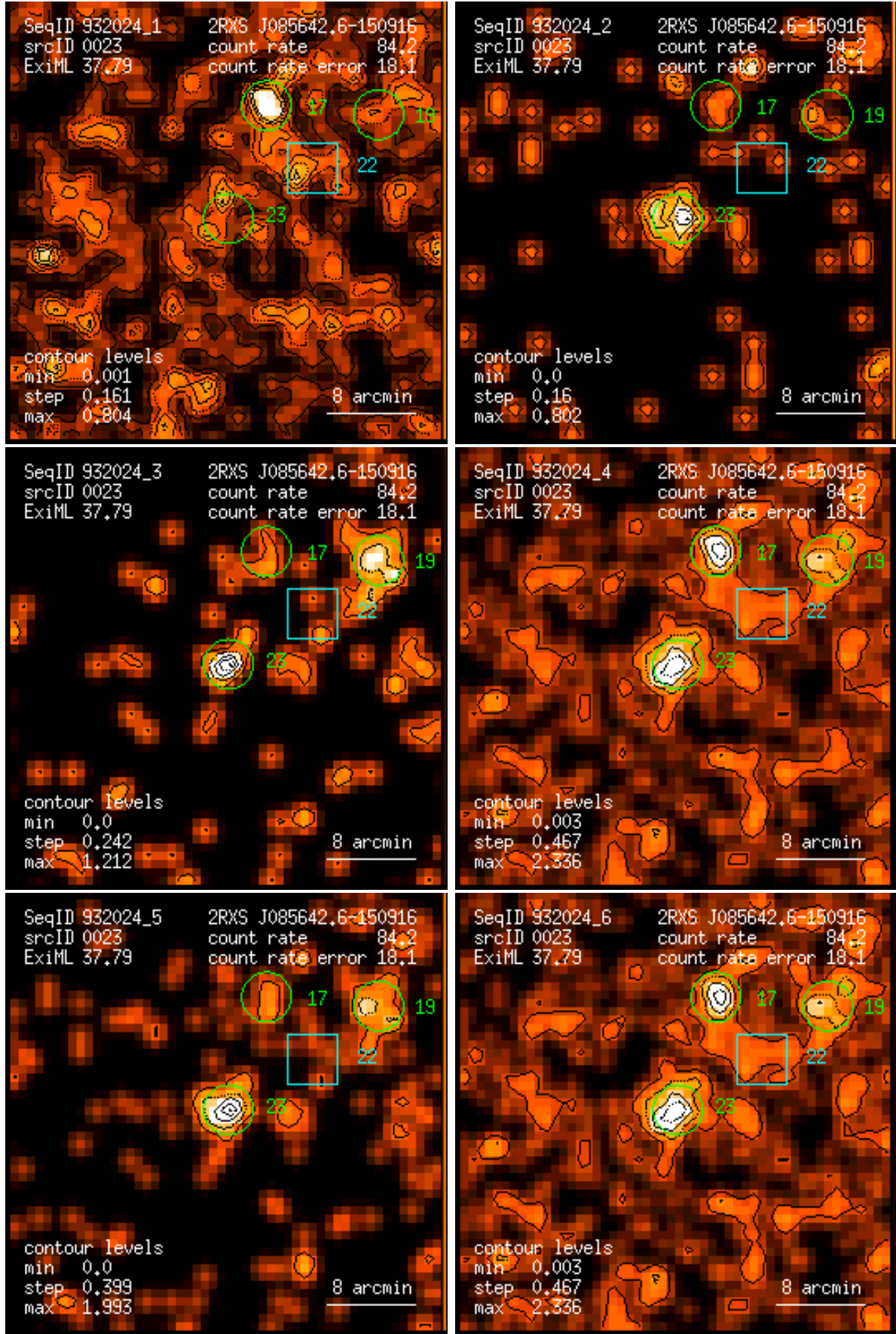
Figure 23: RASS 932024: detection 0023: band rate images, Gaussian filter: (1) PSPC channels 11 – 41, (2) 52 – 90, (3) 91 – 201, (4) 11 – 235, (5) 52 – 201, (6) 11 – 201. Broad band rates in counts/ks. Band rate contour levels in counts/ks/arcmin 2 .
