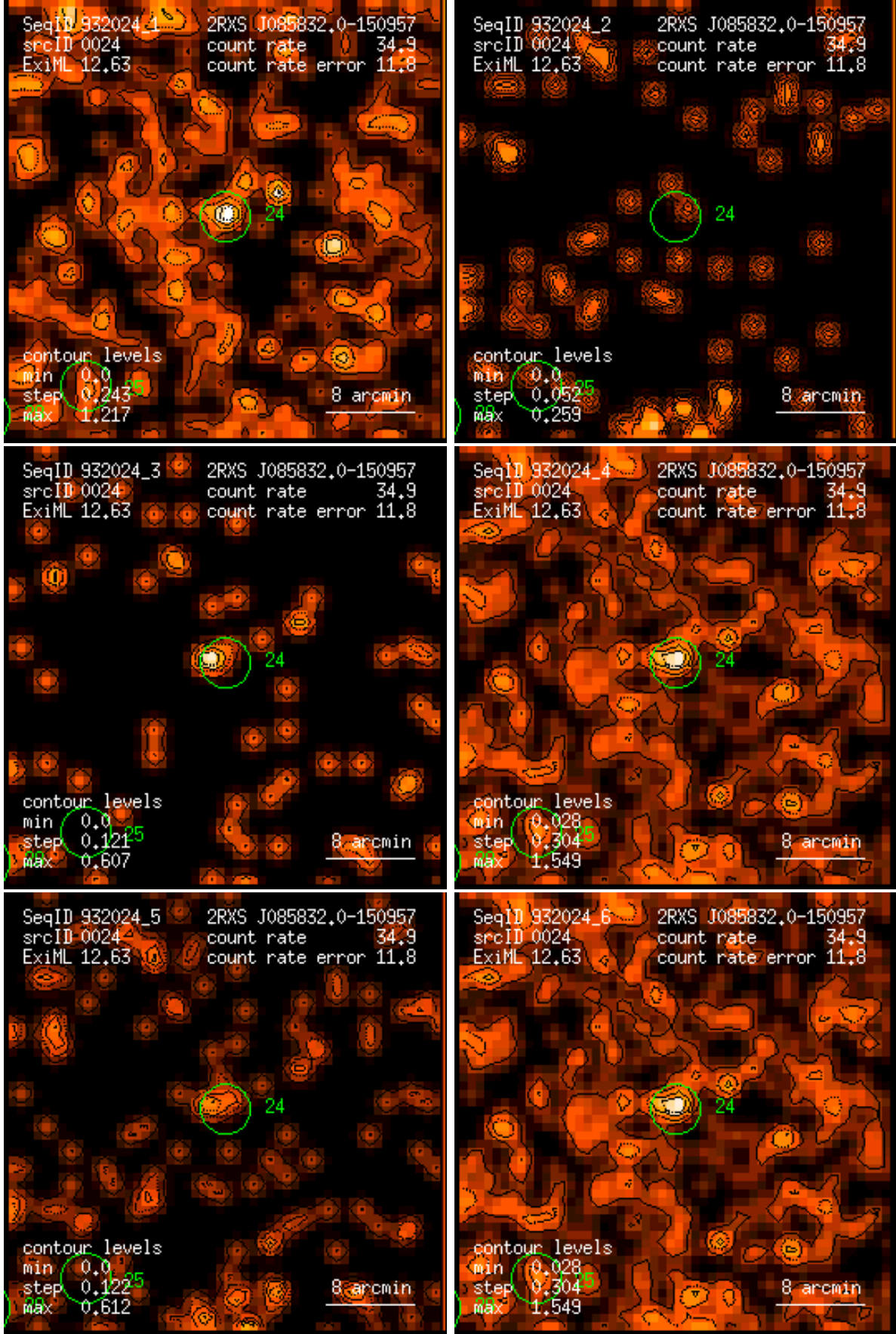
Figure 24: RASS 932024: detection 0024: band rate images, Gaussian filter: (1) PSPC channels 11 – 41, (2) 52 – 90, (3) 91 – 201, (4) 11 – 235, (5) 52 – 201, (6) 11 – 201. Broad band rates in counts/ks. Band rate contour levels in counts/ks/arcmin 2 .
