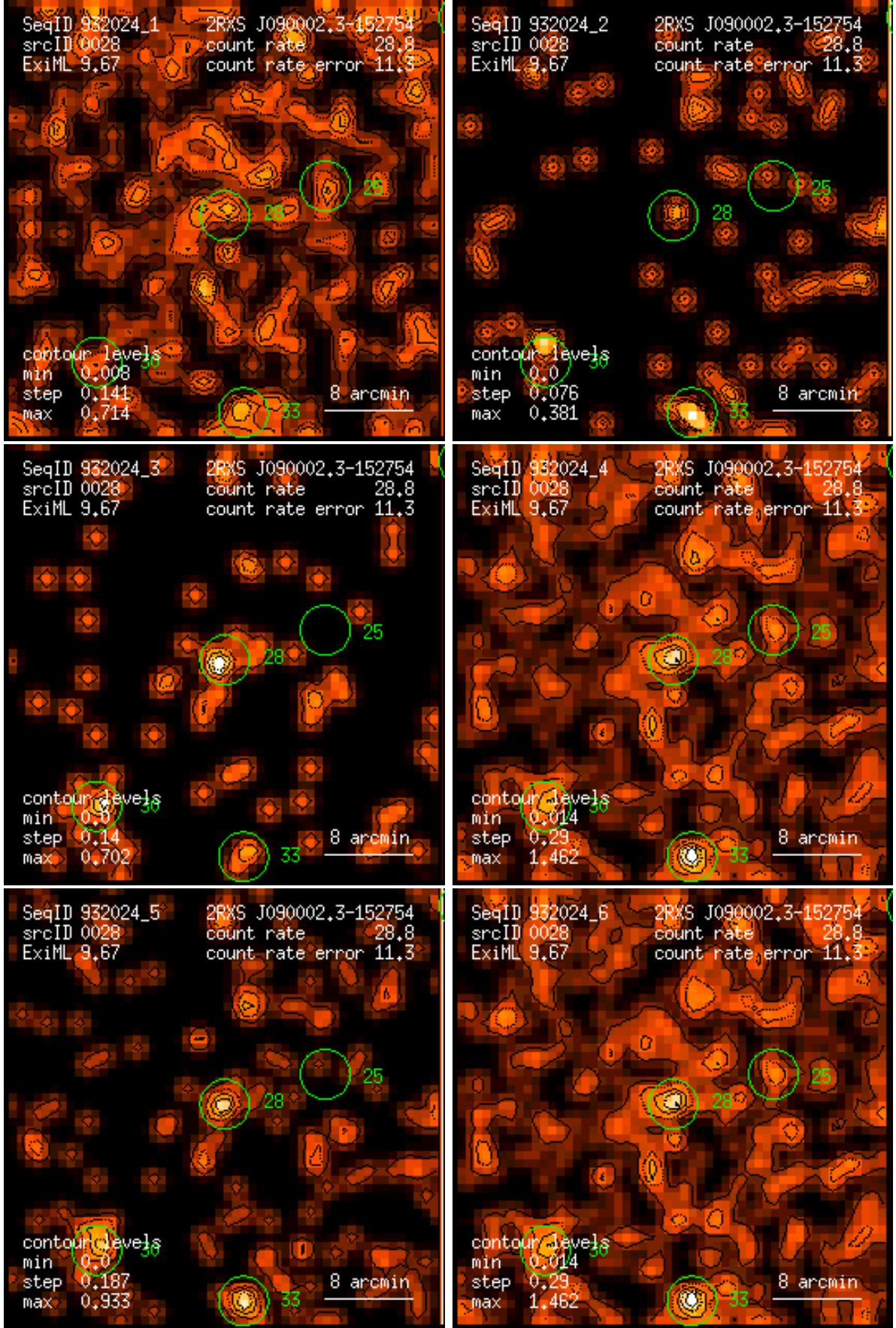
Figure 28: RASS 932024: detection 0028: band rate images, Gaussian filter: (1) PSPC channels 11 – 41, (2) 52 – 90, (3) 91 – 201, (4) 11 – 235, (5) 52 – 201, (6) 11 – 201. Broad band rates in counts/ks. Band rate contour levels in counts/ks/arcmin 2 .
