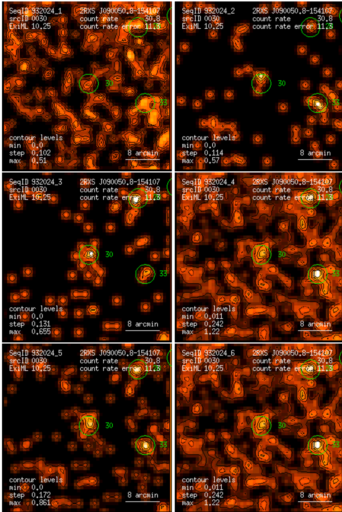
Figure 30: RASS 932024: detection 0030: band rate images, Gaussian filter: (1) PSPC channels 11 – 41, (2) 52 – 90, (3) 91 – 201, (4) 11 – 235, (5) 52 – 201, (6) 11 – 201. Broad band rates in counts/ks. Band rate contour levels in counts/ks/arcmin 2 .
