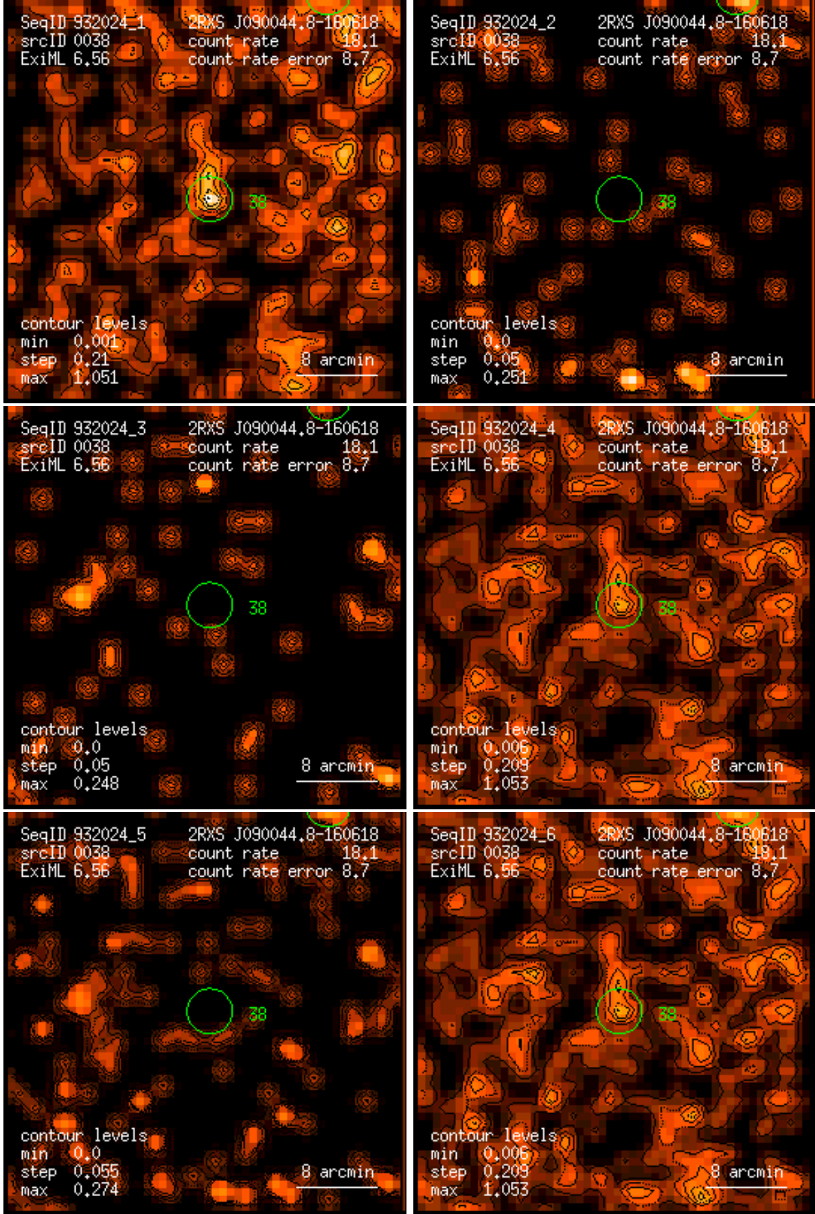
Figure 38: RASS 932024: detection 0038: band rate images, Gaussian filter: (1) PSPC channels 11 – 41, (2) 52 – 90, (3) 91 – 201, (4) 11 – 235, (5) 52 – 201, (6) 11 – 201. Broad band rates in counts/ks. Band rate contour levels in counts/ks/arcmin 2 .
