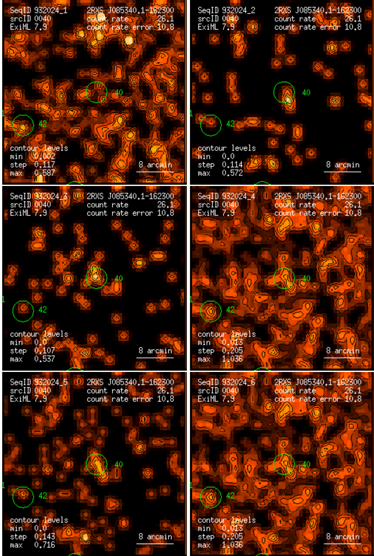
Figure 40: RASS 932024: detection 0040: band rate images, Gaussian filter: (1) PSPC channels 11 – 41, (2) 52 – 90, (3) 91 – 201, (4) 11 – 235, (5) 52 – 201, (6) 11 – 201. Broad band rates in counts/ks. Band rate contour levels in counts/ks/arcmin 2 .
