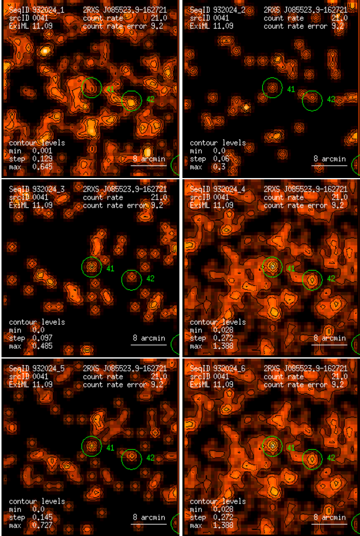
Figure 41: RASS 932024: detection 0041: band rate images, Gaussian filter: (1) PSPC channels 11 – 41, (2) 52 – 90, (3) 91 – 201, (4) 11 – 235, (5) 52 – 201, (6) 11 – 201. Broad band rates in counts/ks. Band rate contour levels in counts/ks/arcmin 2 .
