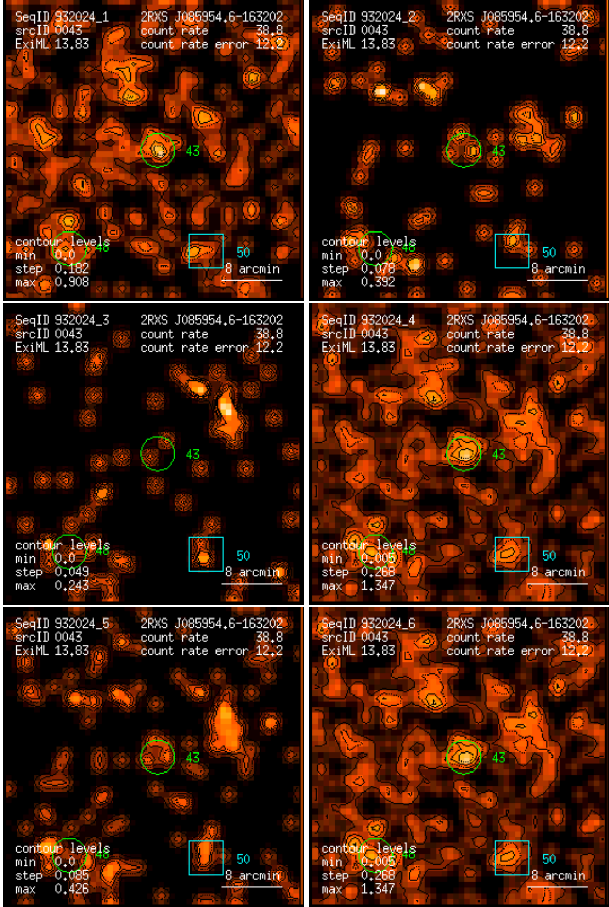
Figure 43: RASS 932024: detection 0043: band rate images, Gaussian filter: (1) PSPC channels 11 – 41, (2) 52 – 90, (3) 91 – 201, (4) 11 – 235, (5) 52 – 201, (6) 11 – 201. Broad band rates in counts/ks. Band rate contour levels in counts/ks/arcmin 2 .
