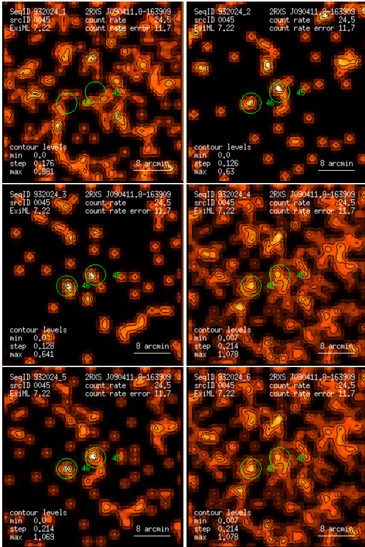
Figure 45: RASS 932024: detection 0045: band rate images, Gaussian filter: (1) PSPC channels 11 – 41, (2) 52 – 90, (3) 91 – 201, (4) 11 – 235, (5) 52 – 201, (6) 11 – 201. Broad band rates in counts/ks. Band rate contour levels in counts/ks/arcmin 2 .
