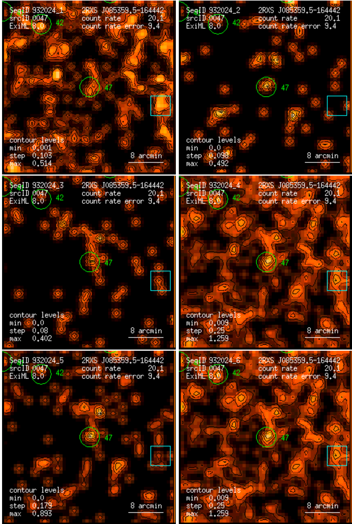
Figure 47: RASS 932024: detection 0047: band rate images, Gaussian filter: (1) PSPC channels 11 – 41, (2) 52 – 90, (3) 91 – 201, (4) 11 – 235, (5) 52 – 201, (6) 11 – 201. Broad band rates in counts/ks. Band rate contour levels in counts/ks/arcmin 2 .
