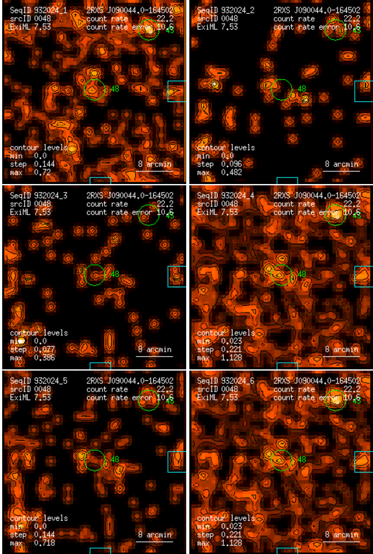
Figure 48: RASS 932024: detection 0048: band rate images, Gaussian filter: (1) PSPC channels 11 – 41, (2) 52 – 90, (3) 91 – 201, (4) 11 – 235, (5) 52 – 201, (6) 11 – 201. Broad band rates in counts/ks. Band rate contour levels in counts/ks/arcmin 2 .
