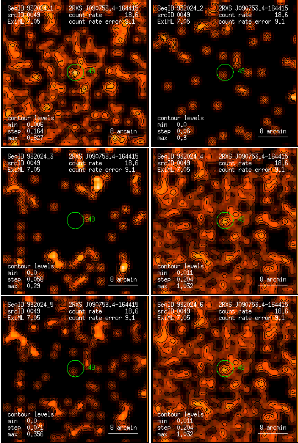
Figure 49: RASS 932024: detection 0049: band rate images, Gaussian filter: (1) PSPC channels 11 – 41, (2) 52 – 90, (3) 91 – 201, (4) 11 – 235, (5) 52 – 201, (6) 11 – 201. Broad band rates in counts/ks. Band rate contour levels in counts/ks/arcmin 2 .
