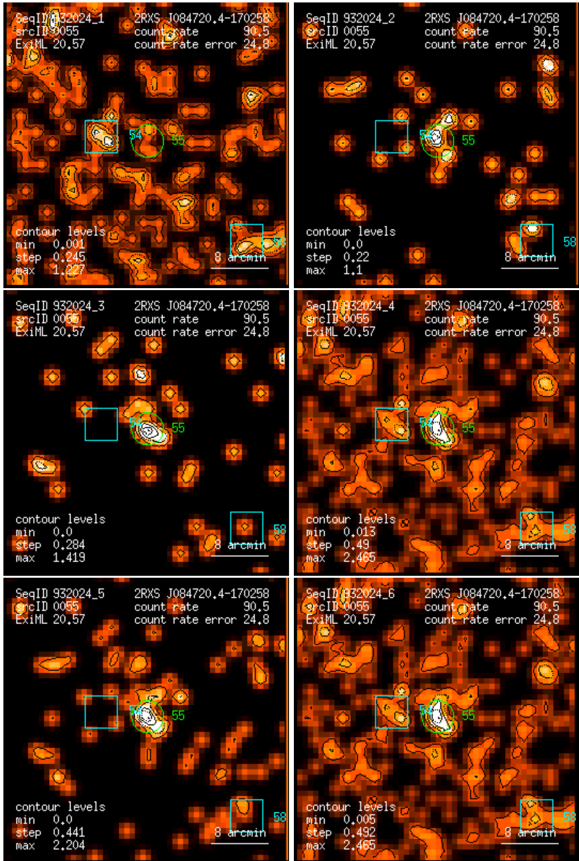
Figure 55: RASS 932024: detection 0055: band rate images, Gaussian filter: (1) PSPC channels 11 – 41, (2) 52 – 90, (3) 91 – 201, (4) 11 – 235, (5) 52 – 201, (6) 11 – 201. Broad band rates in counts/ks. Band rate contour levels in counts/ks/arcmin 2 .
