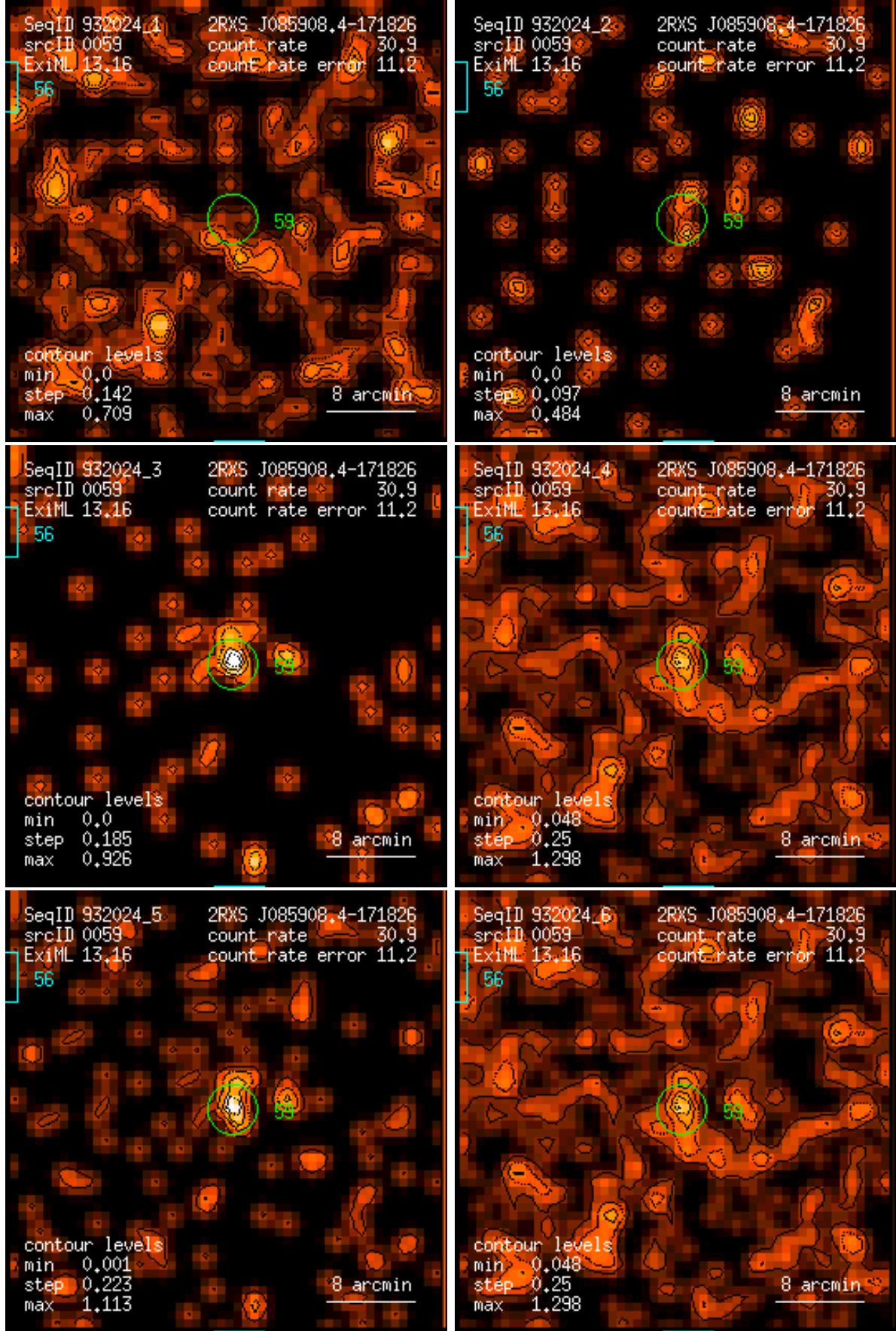
Figure 59: RASS 932024: detection 0059: band rate images, Gaussian filter: (1) PSPC channels 11 – 41, (2) 52 – 90, (3) 91 – 201, (4) 11 – 235, (5) 52 – 201, (6) 11 – 201. Broad band rates in counts/ks. Band rate contour levels in counts/ks/arcmin 2 .
