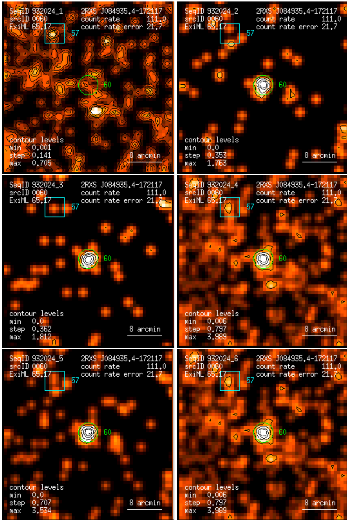
Figure 60: RASS 932024: detection 0060: band rate images, Gaussian filter: (1) PSPC channels 11 – 41, (2) 52 – 90, (3) 91 – 201, (4) 11 – 235, (5) 52 – 201, (6) 11 – 201. Broad band rates in counts/ks. Band rate contour levels in counts/ks/arcmin 2 .
