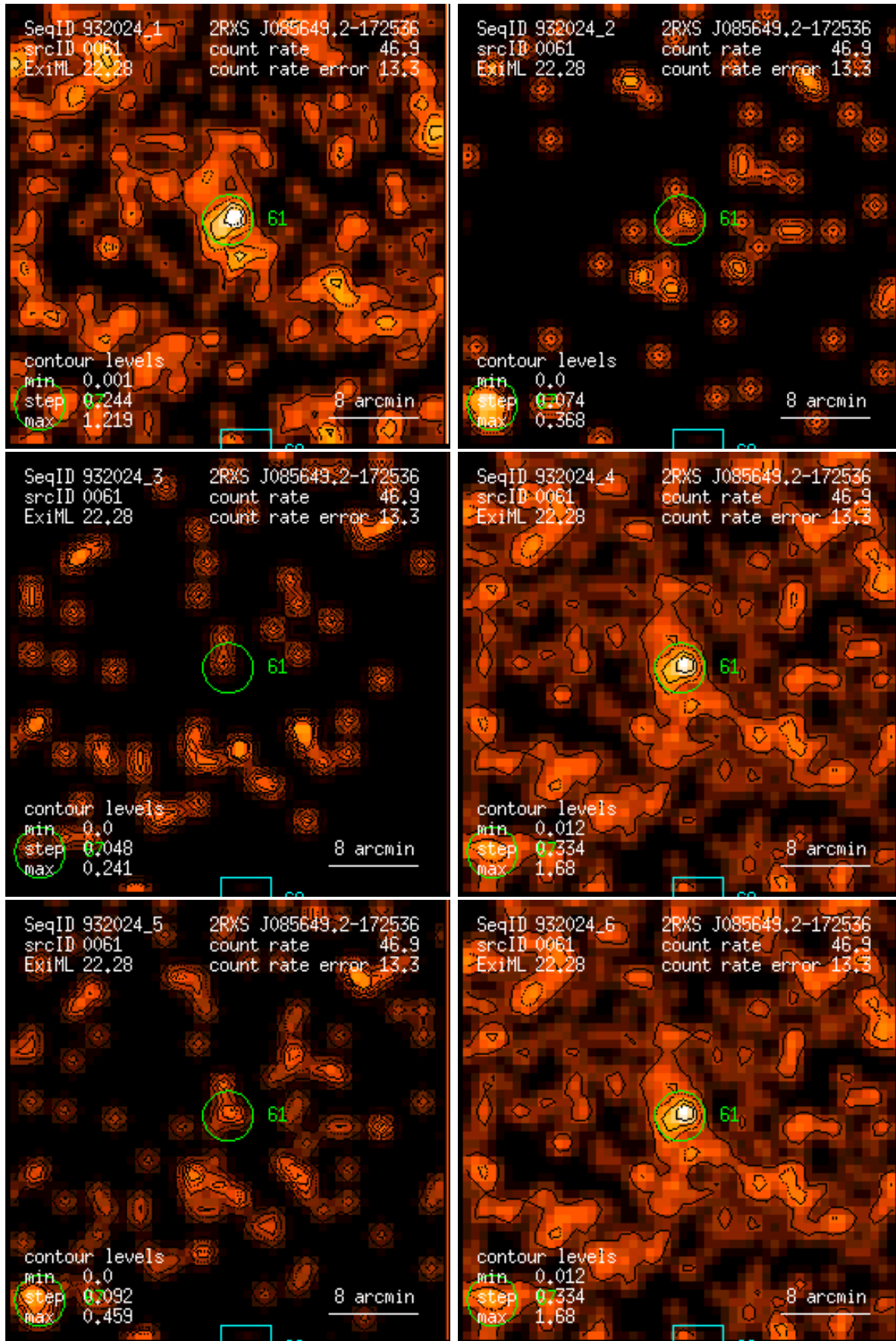
Figure 61: RASS 932024: detection 0061: band rate images, Gaussian filter: (1) PSPC channels 11 – 41, (2) 52 – 90, (3) 91 – 201, (4) 11 – 235, (5) 52 – 201, (6) 11 – 201. Broad band rates in counts/ks. Band rate contour levels in counts/ks/arcmin 2 .
