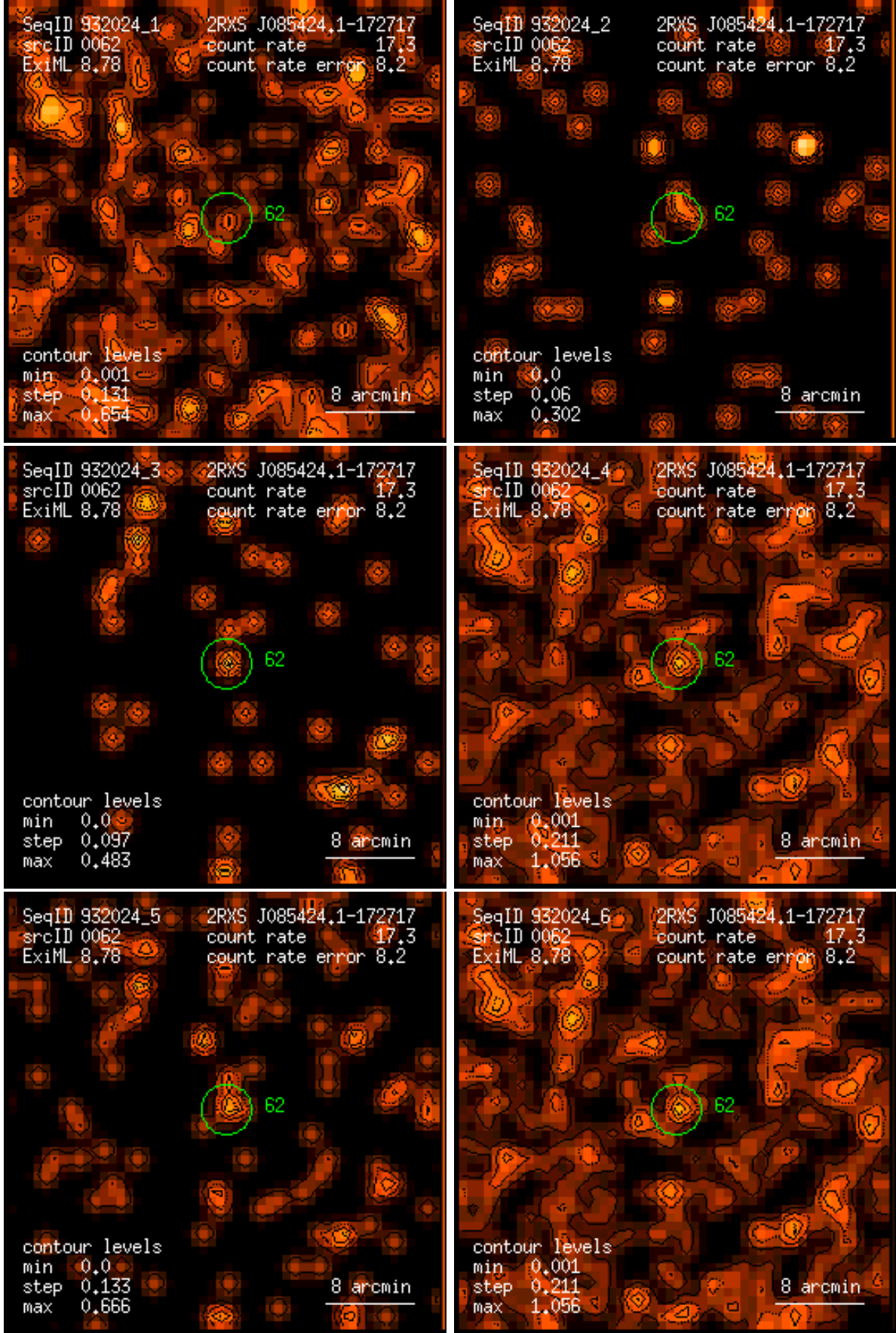
Figure 62: RASS 932024: detection 0062: band rate images, Gaussian filter: (1) PSPC channels 11 – 41, (2) 52 – 90, (3) 91 – 201, (4) 11 – 235, (5) 52 – 201, (6) 11 – 201. Broad band rates in counts/ks. Band rate contour levels in counts/ks/arcmin 2 .
