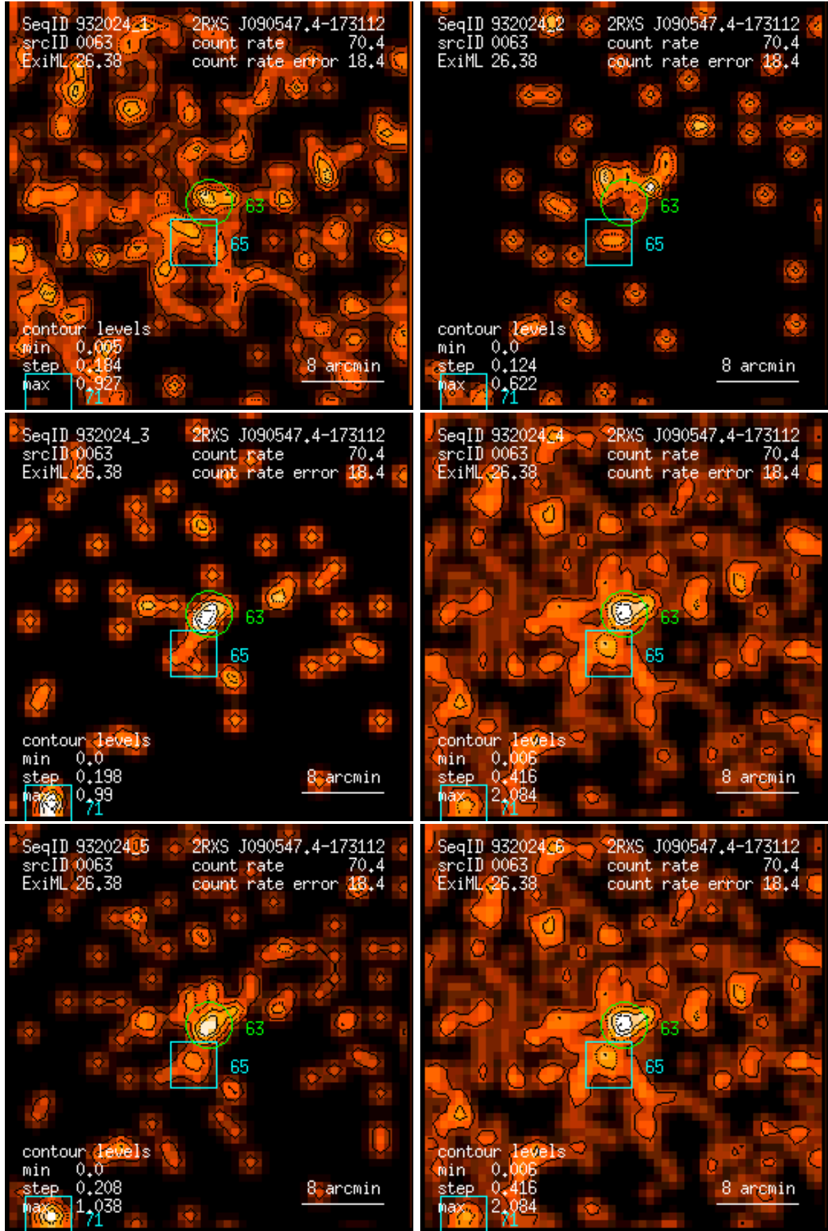
Figure 63: RASS 932024: detection 0063: band rate images, Gaussian filter: (1) PSPC channels 11 – 41, (2) 52 – 90, (3) 91 – 201, (4) 11 – 235, (5) 52 – 201, (6) 11 – 201. Broad band rates in counts/ks. Band rate contour levels in counts/ks/arcmin 2 .
