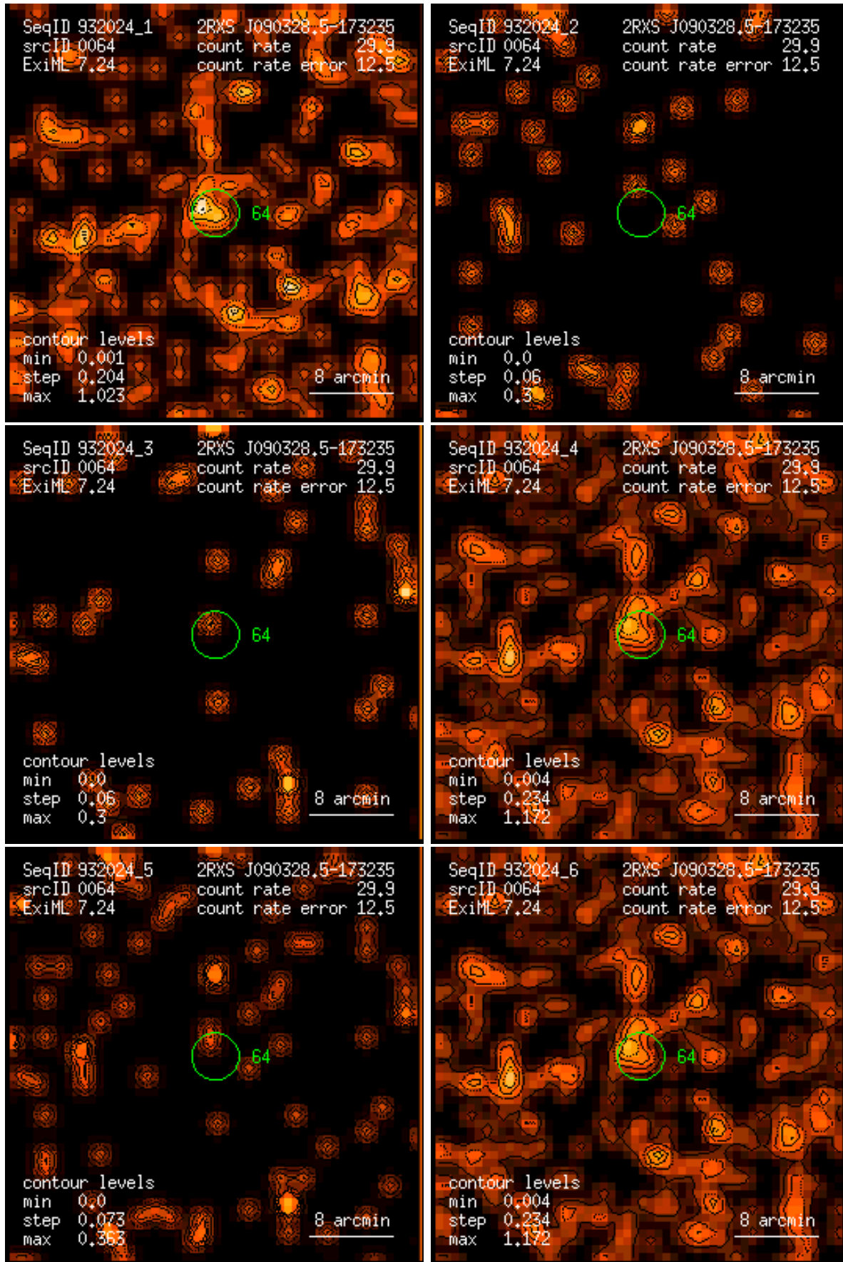
Figure 64: RASS 932024: detection 0064: band rate images, Gaussian filter: (1) PSPC channels 11 – 41, (2) 52 – 90, (3) 91 – 201, (4) 11 – 235, (5) 52 – 201, (6) 11 – 201. Broad band rates in counts/ks. Band rate contour levels in counts/ks/arcmin 2 .
