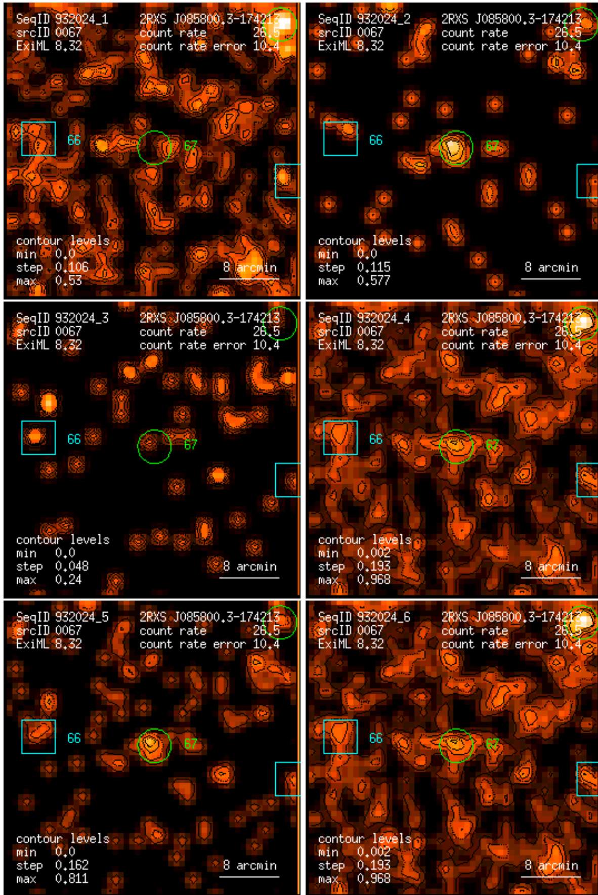
Figure 67: RASS 932024: detection 0067: band rate images, Gaussian filter: (1) PSPC channels 11 – 41, (2) 52 – 90, (3) 91 – 201, (4) 11 – 235, (5) 52 – 201, (6) 11 – 201. Broad band rates in counts/ks. Band rate contour levels in counts/ks/arcmin 2 .
