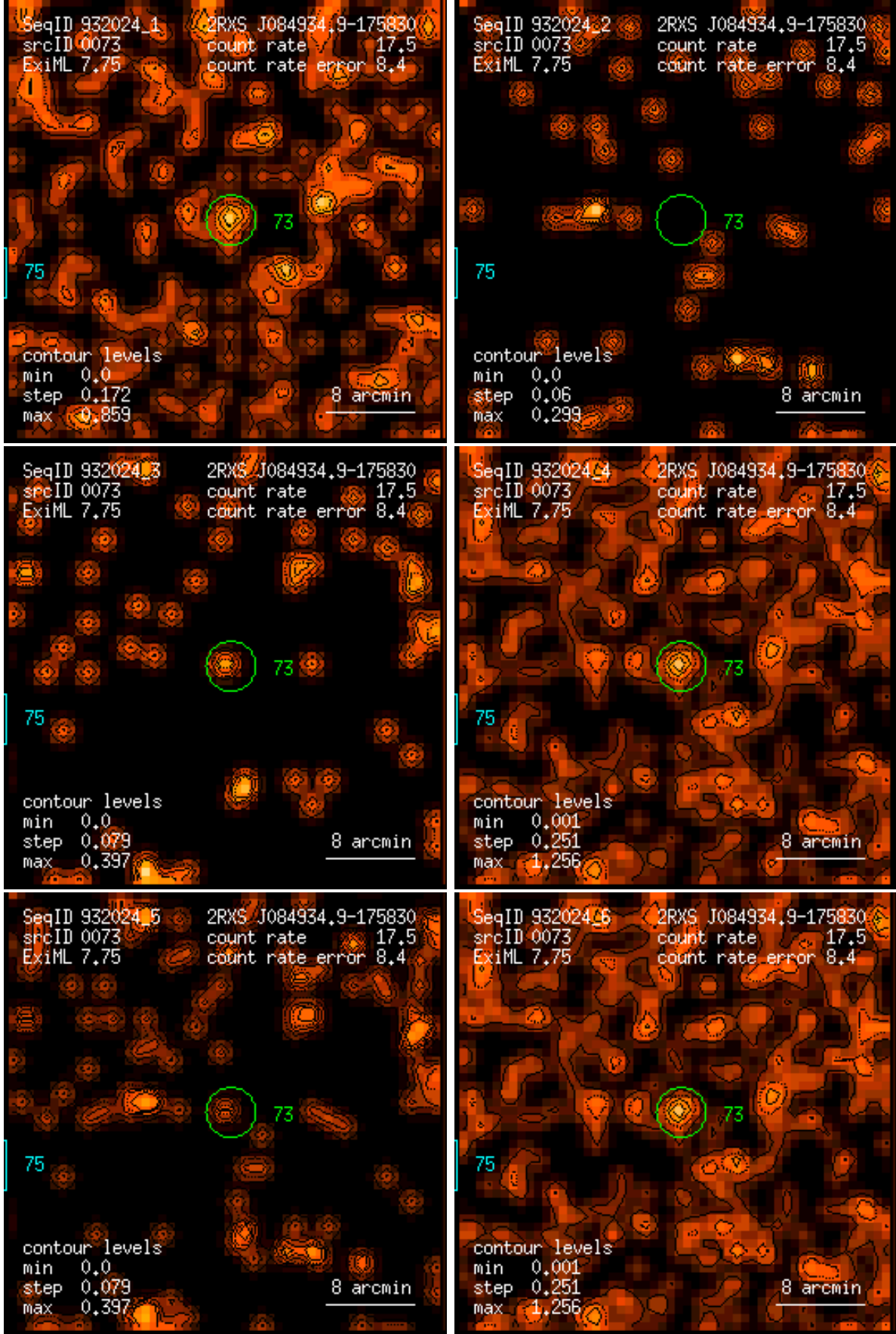
Figure 73: RASS 932024: detection 0073: band rate images, Gaussian filter: (1) PSPC channels 11 – 41, (2) 52 – 90, (3) 91 – 201, (4) 11 – 235, (5) 52 – 201, (6) 11 – 201. Broad band rates in counts/ks. Band rate contour levels in counts/ks/arcmin 2 .
