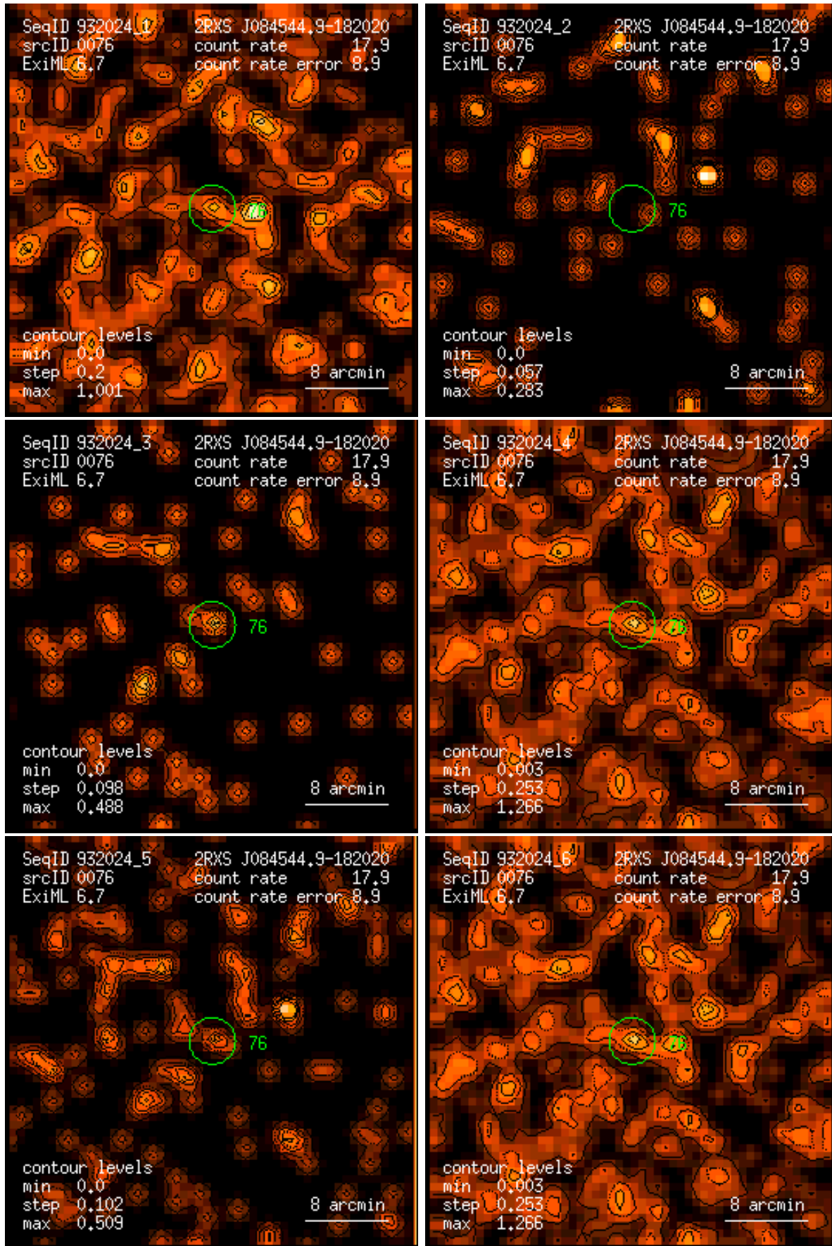
Figure 76: RASS 932024: detection 0076: band rate images, Gaussian filter: (1) PSPC channels 11 – 41, (2) 52 – 90, (3) 91 – 201, (4) 11 – 235, (5) 52 – 201, (6) 11 – 201. Broad band rates in counts/ks. Band rate contour levels in counts/ks/arcmin 2 .
