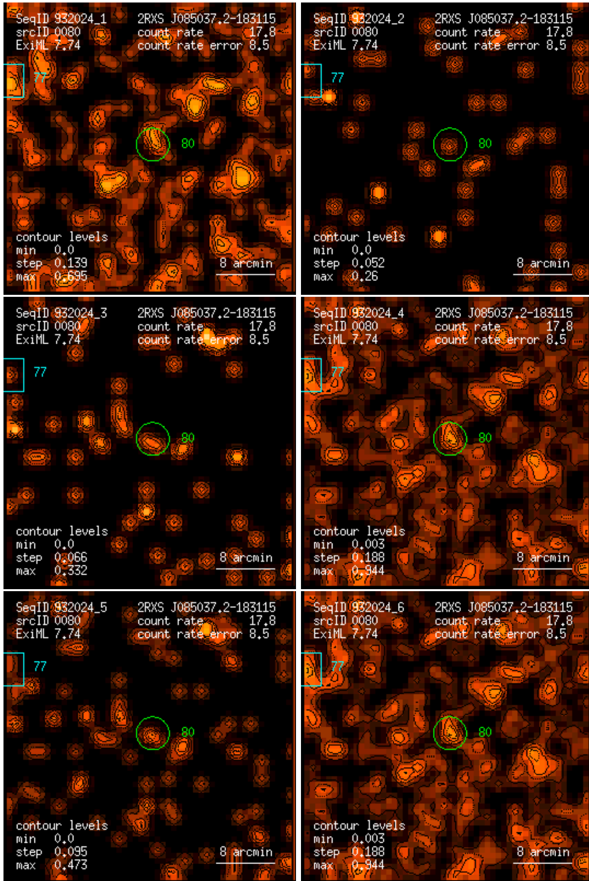
Figure 80: RASS 932024: detection 0080: band rate images, Gaussian filter: (1) PSPC channels 11 – 41, (2) 52 – 90, (3) 91 – 201, (4) 11 – 235, (5) 52 – 201, (6) 11 – 201. Broad band rates in counts/ks. Band rate contour levels in counts/ks/arcmin 2 .
