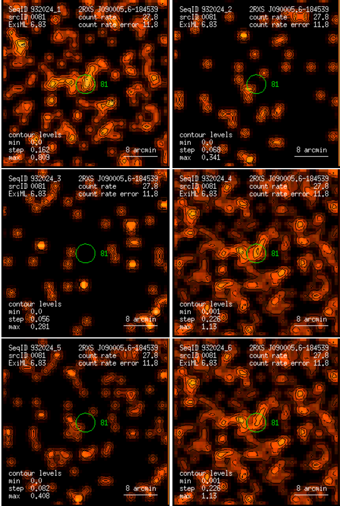
Figure 81: RASS 932024: detection 0081: band rate images, Gaussian filter: (1) PSPC channels 11 – 41, (2) 52 – 90, (3) 91 – 201, (4) 11 – 235, (5) 52 – 201, (6) 11 – 201. Broad band rates in counts/ks. Band rate contour levels in counts/ks/arcmin 2 .
