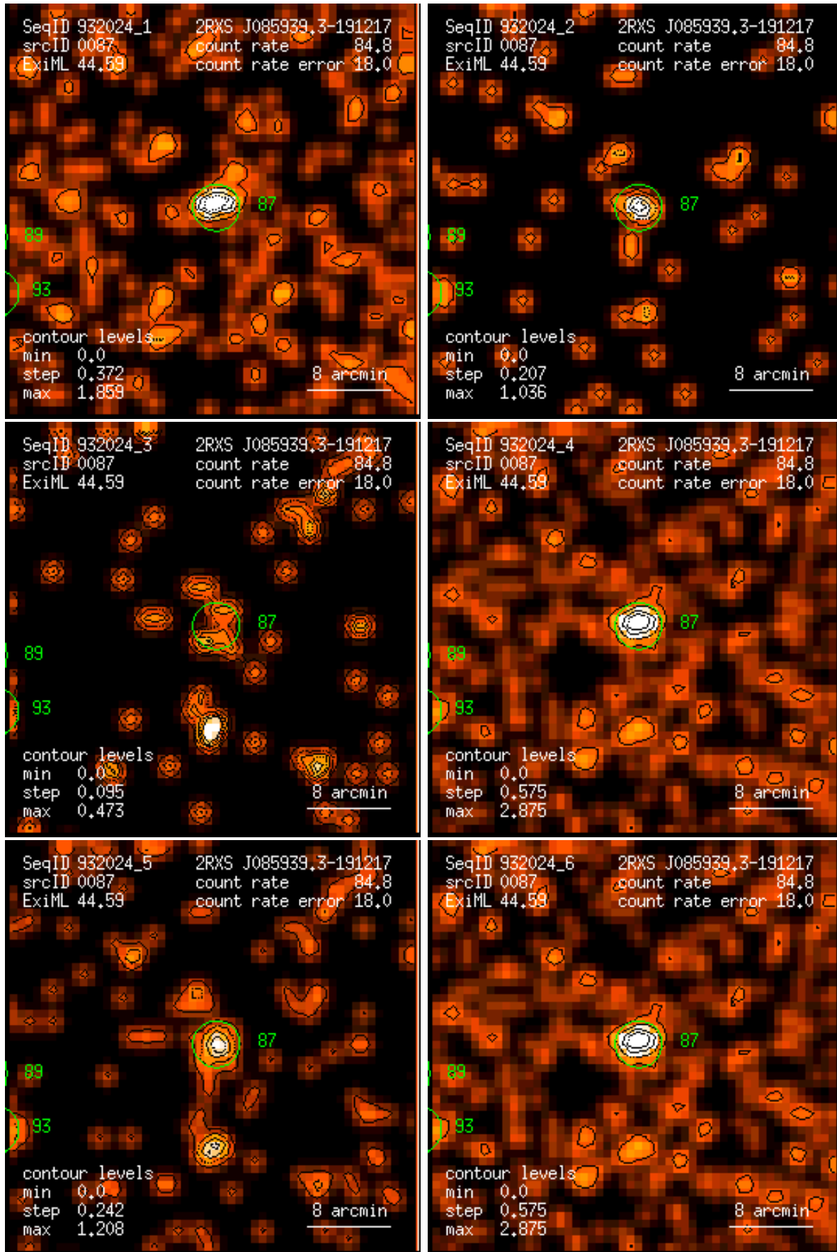
Figure 87: RASS 932024: detection 0087: band rate images, Gaussian filter: (1) PSPC channels 11 – 41, (2) 52 – 90, (3) 91 – 201, (4) 11 – 235, (5) 52 – 201, (6) 11 – 201. Broad band rates in counts/ks. Band rate contour levels in counts/ks/arcmin 2 .
