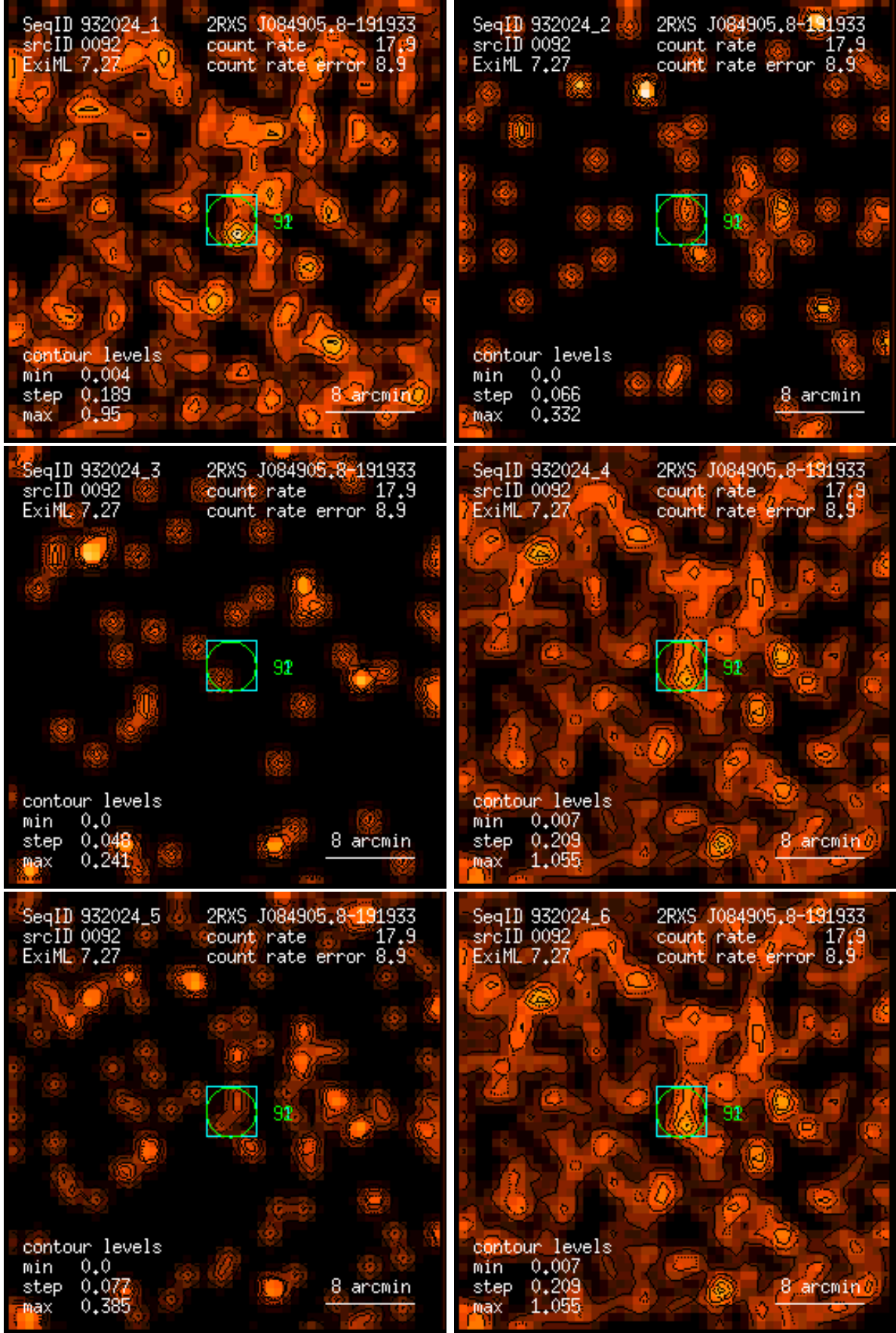
Figure 92: RASS 932024: detection 0092: band rate images, Gaussian filter: (1) PSPC channels 11 – 41, (2) 52 – 90, (3) 91 – 201, (4) 11 – 235, (5) 52 – 201, (6) 11 – 201. Broad band rates in counts/ks. Band rate contour levels in counts/ks/arcmin 2 .
