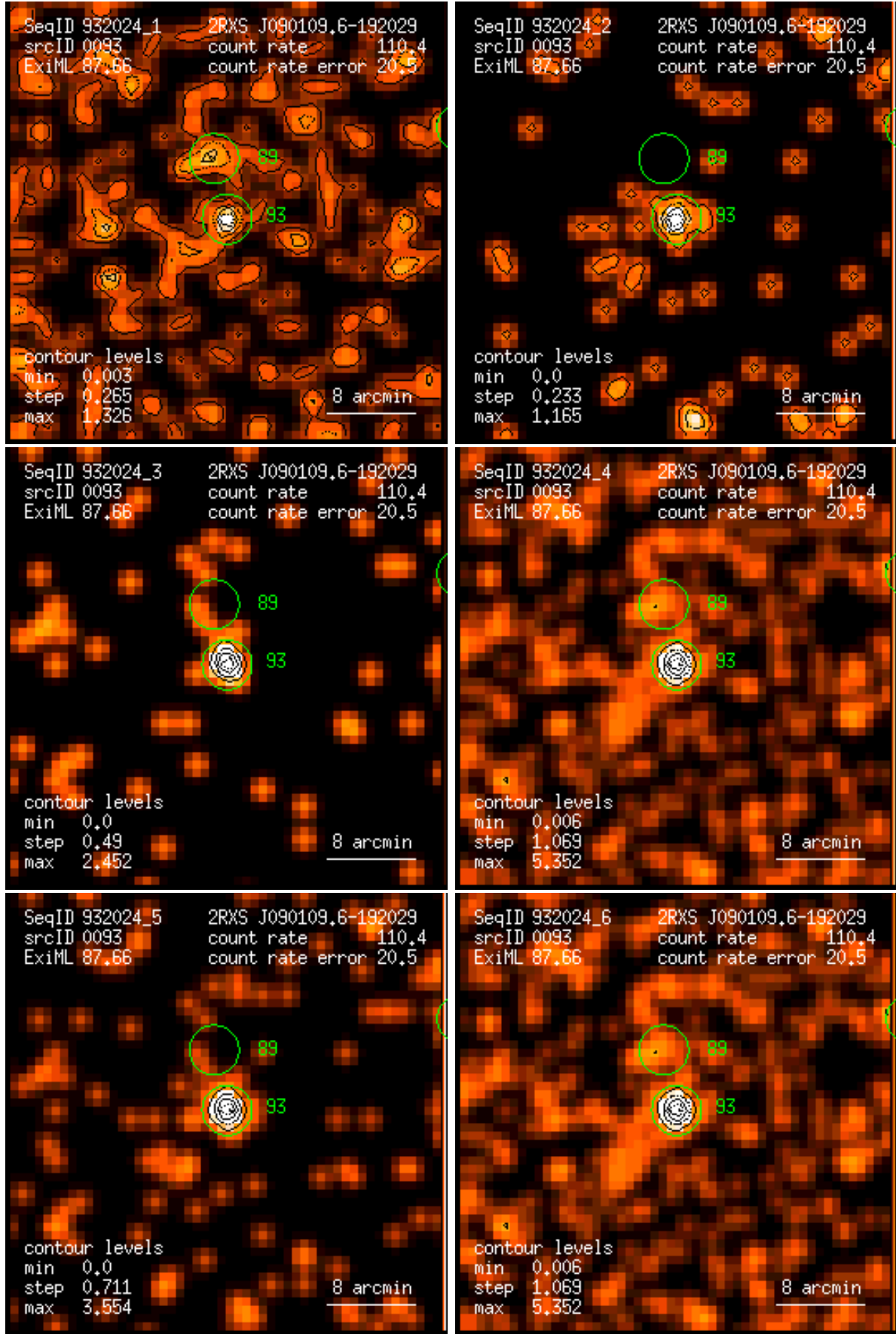
Figure 93: RASS 932024: detection 0093: band rate images, Gaussian filter: (1) PSPC channels 11 – 41, (2) 52 – 90, (3) 91 – 201, (4) 11 – 235, (5) 52 – 201, (6) 11 – 201. Broad band rates in counts/ks. Band rate contour levels in counts/ks/arcmin 2 .
