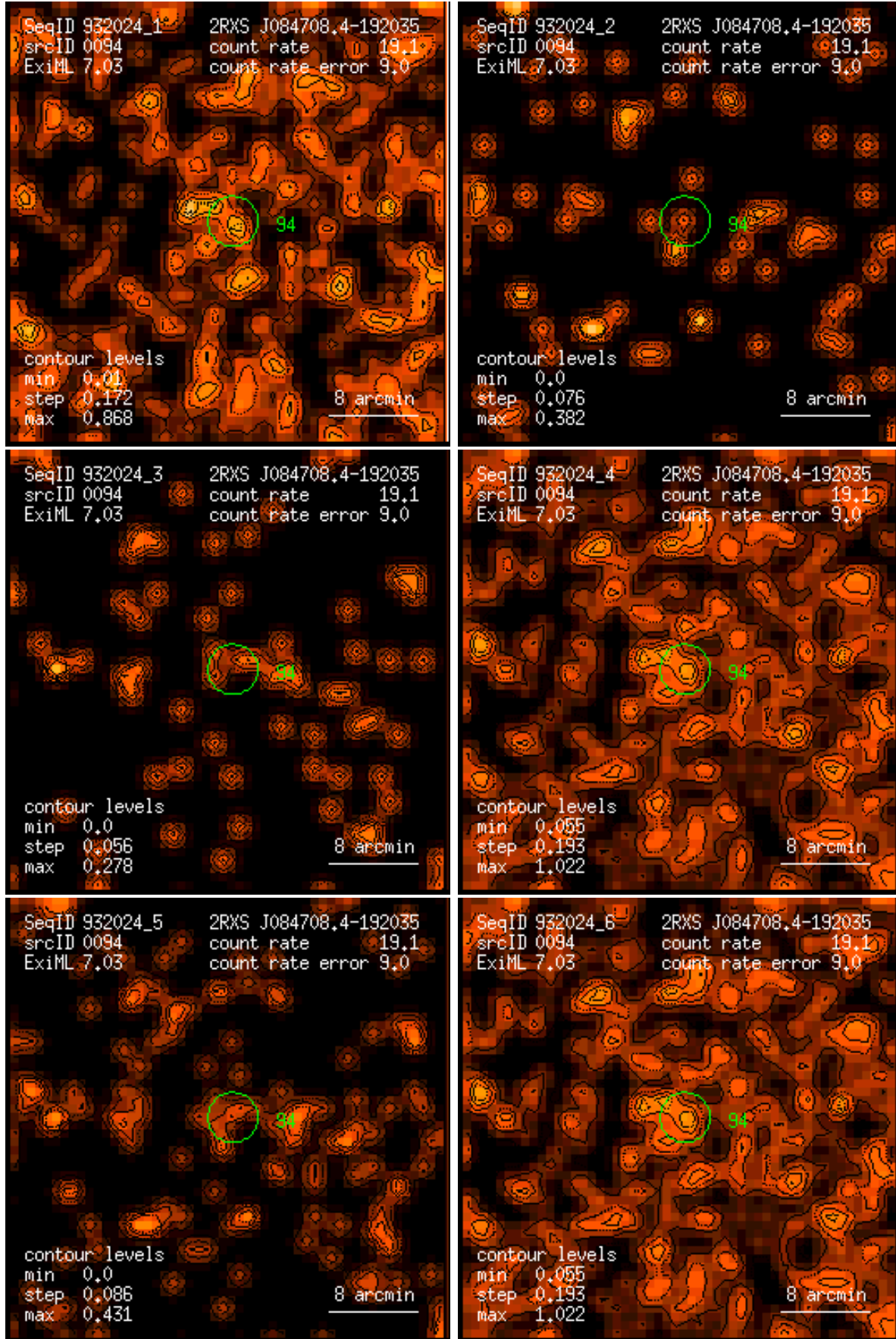
Figure 94: RASS 932024: detection 0094: band rate images, Gaussian filter: (1) PSPC channels 11 – 41, (2) 52 – 90, (3) 91 – 201, (4) 11 – 235, (5) 52 – 201, (6) 11 – 201. Broad band rates in counts/ks. Band rate contour levels in counts/ks/arcmin 2 .
