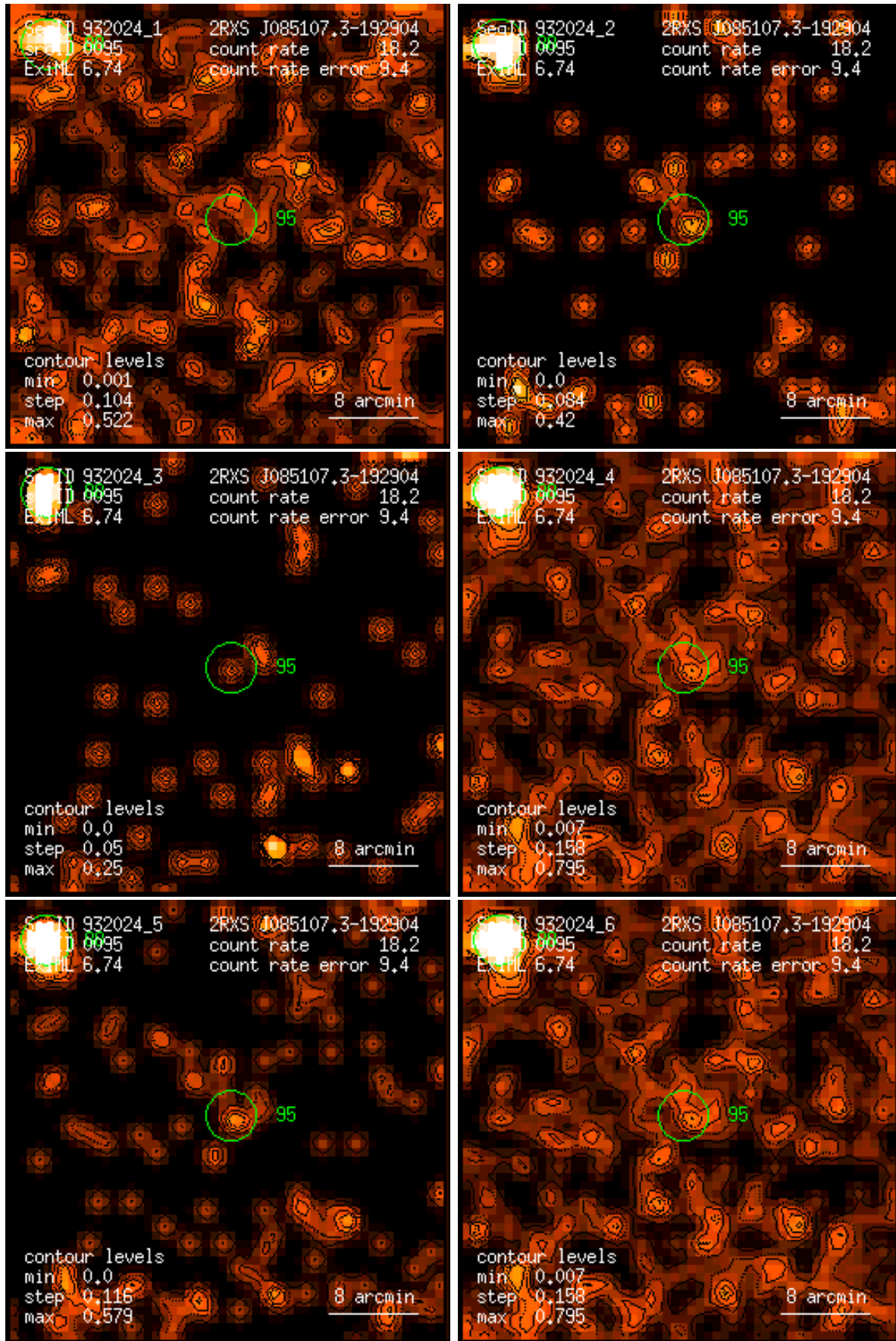
Figure 95: RASS 932024: detection 0095: band rate images, Gaussian filter: (1) PSPC channels 11 – 41, (2) 52 – 90, (3) 91 – 201, (4) 11 – 235, (5) 52 – 201, (6) 11 – 201. Broad band rates in counts/ks. Band rate contour levels in counts/ks/arcmin 2 .
