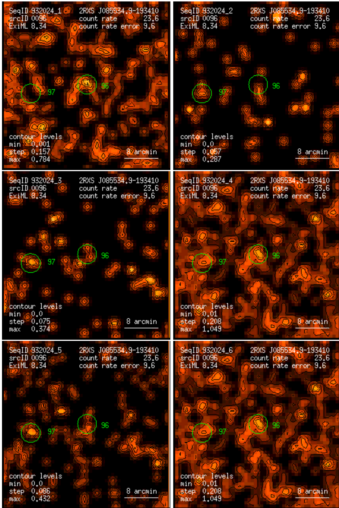
Figure 96: RASS 932024: detection 0096: band rate images, Gaussian filter: (1) PSPC channels 11 – 41, (2) 52 – 90, (3) 91 – 201, (4) 11 – 235, (5) 52 – 201, (6) 11 – 201. Broad band rates in counts/ks. Band rate contour levels in counts/ks/arcmin 2 .
