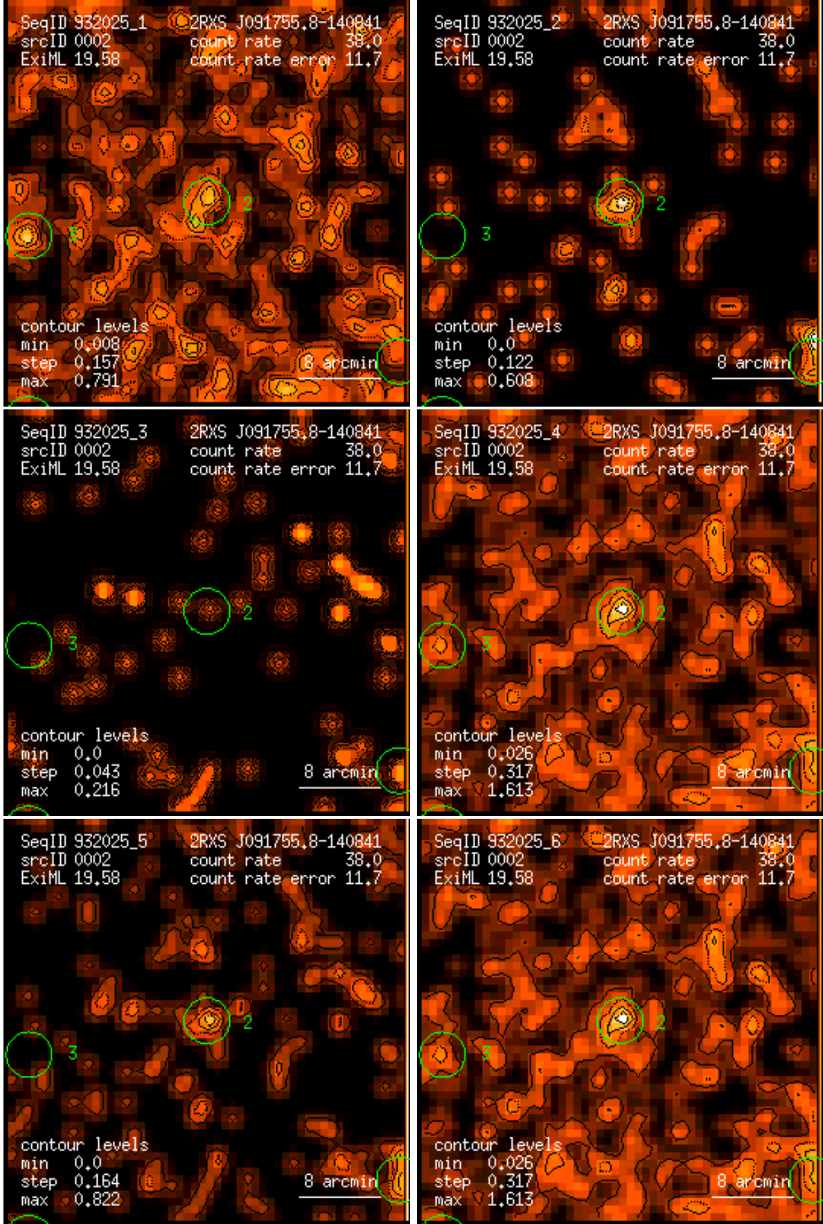
Figure 2: RASS 932025: detection 0002: band rate images, Gaussian filter: (1) PSPC channels 11 – 41, (2) 52 – 90, (3) 91 – 201, (4) 11 – 235, (5) 52 – 201, (6) 11 – 201. Broad band rates in counts/ks. Band rate contour levels in counts/ks/arcmin 2 .
