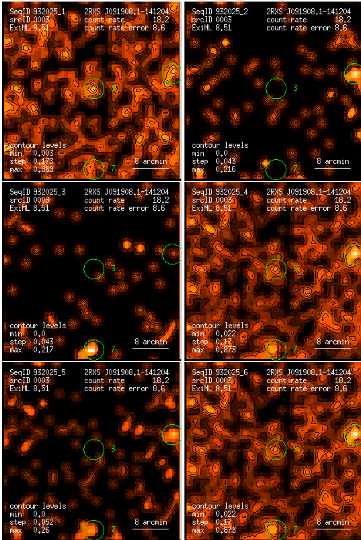
Figure 3: RASS 932025: detection 0003: band rate images, Gaussian filter: (1) PSPC channels 11 – 41, (2) 52 – 90, (3) 91 – 201, (4) 11 – 235, (5) 52 – 201, (6) 11 – 201. Broad band rates in counts/ks. Band rate contour levels in counts/ks/arcmin 2 .
