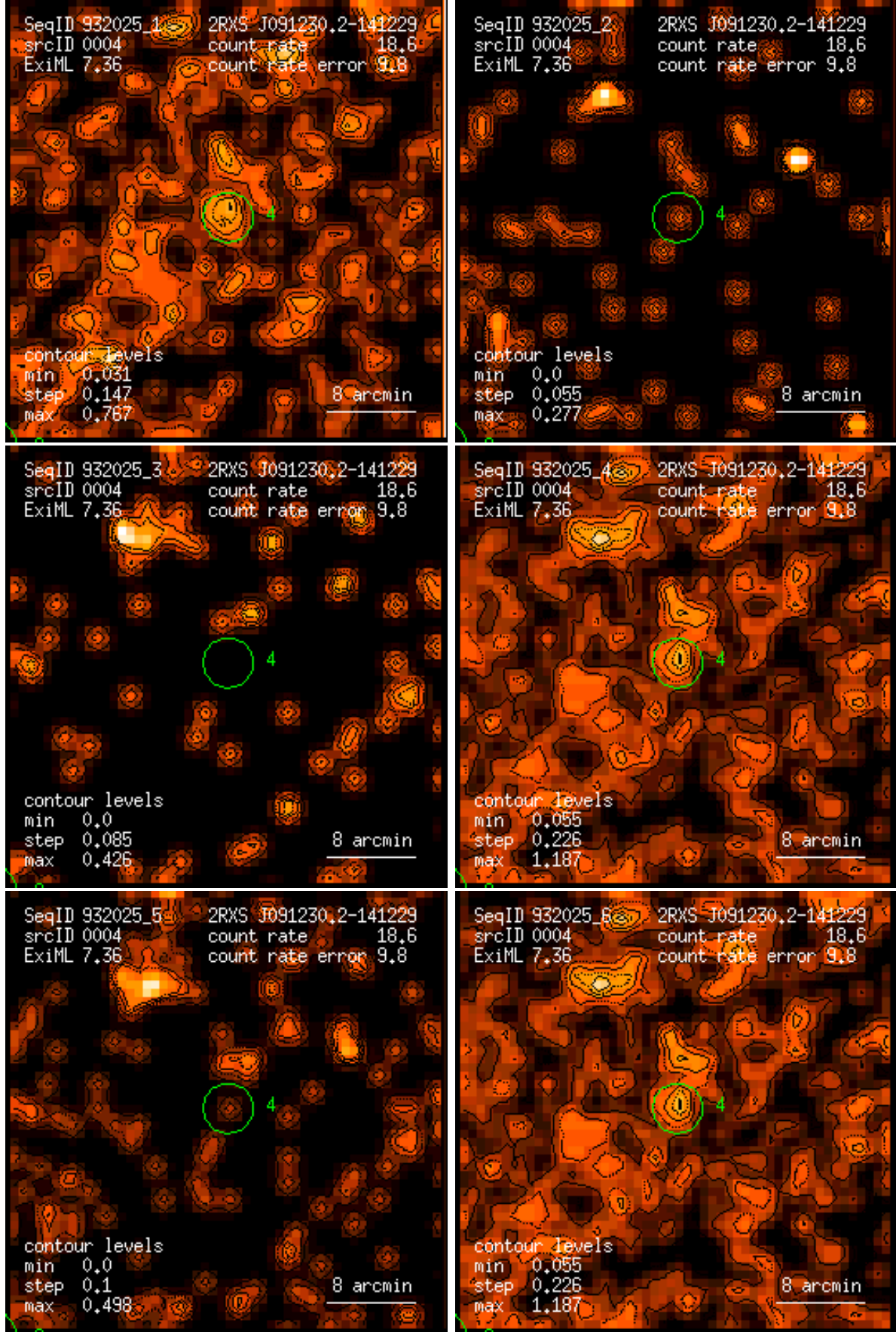
Figure 4: RASS 932025: detection 0004: band rate images, Gaussian filter: (1) PSPC channels 11 – 41, (2) 52 – 90, (3) 91 – 201, (4) 11 – 235, (5) 52 – 201, (6) 11 – 201. Broad band rates in counts/ks. Band rate contour levels in counts/ks/arcmin 2 .
