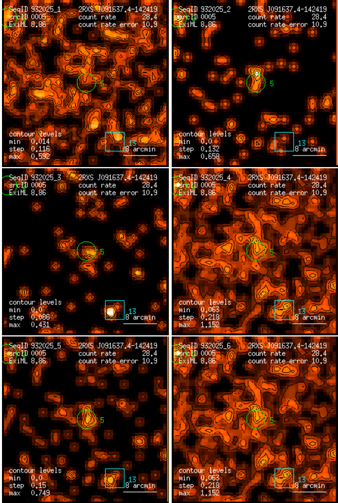
Figure 5: RASS 932025: detection 0005: band rate images, Gaussian filter: (1) PSPC channels 11 – 41, (2) 52 – 90, (3) 91 – 201, (4) 11 – 235, (5) 52 – 201, (6) 11 – 201. Broad band rates in counts/ks. Band rate contour levels in counts/ks/arcmin 2 .
