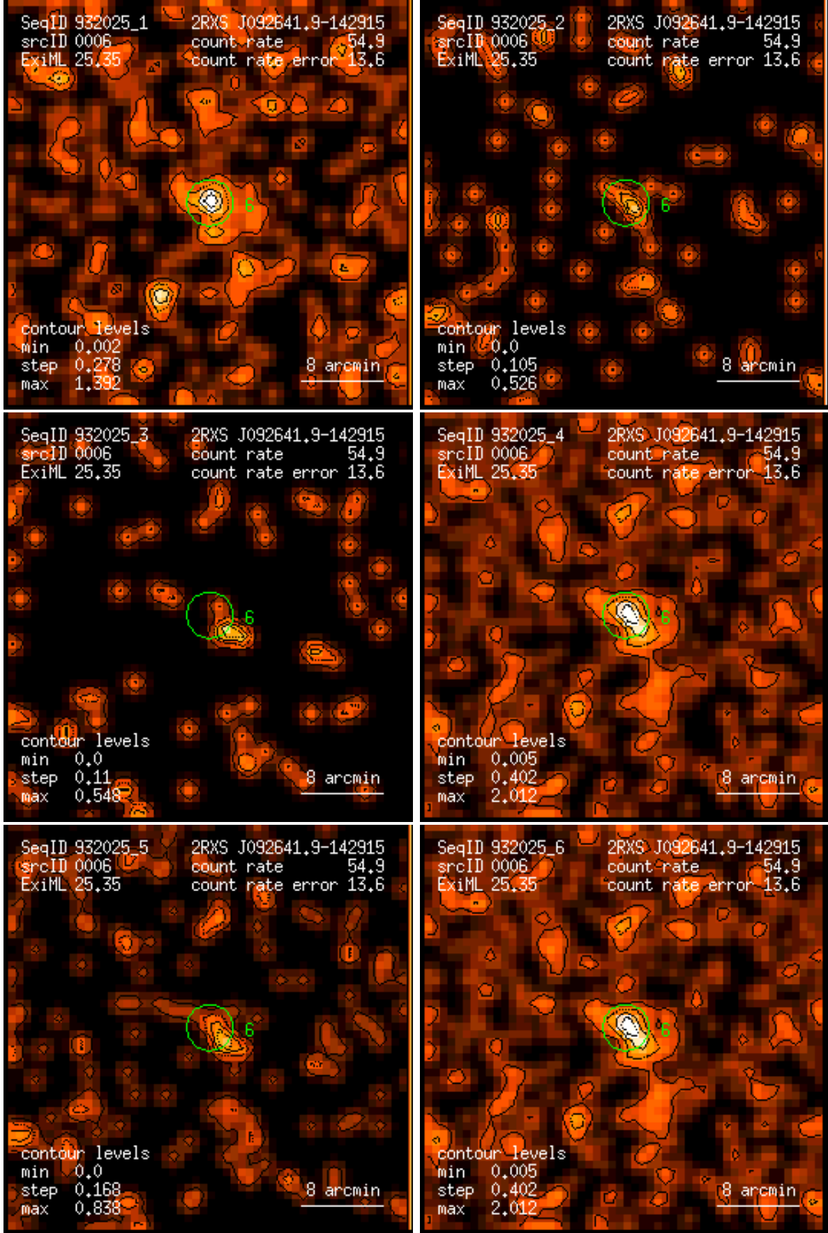
Figure 6: RASS 932025: detection 0006: band rate images, Gaussian filter: (1) PSPC channels 11 – 41, (2) 52 – 90, (3) 91 – 201, (4) 11 – 235, (5) 52 – 201, (6) 11 – 201. Broad band rates in counts/ks. Band rate contour levels in counts/ks/arcmin 2 .
