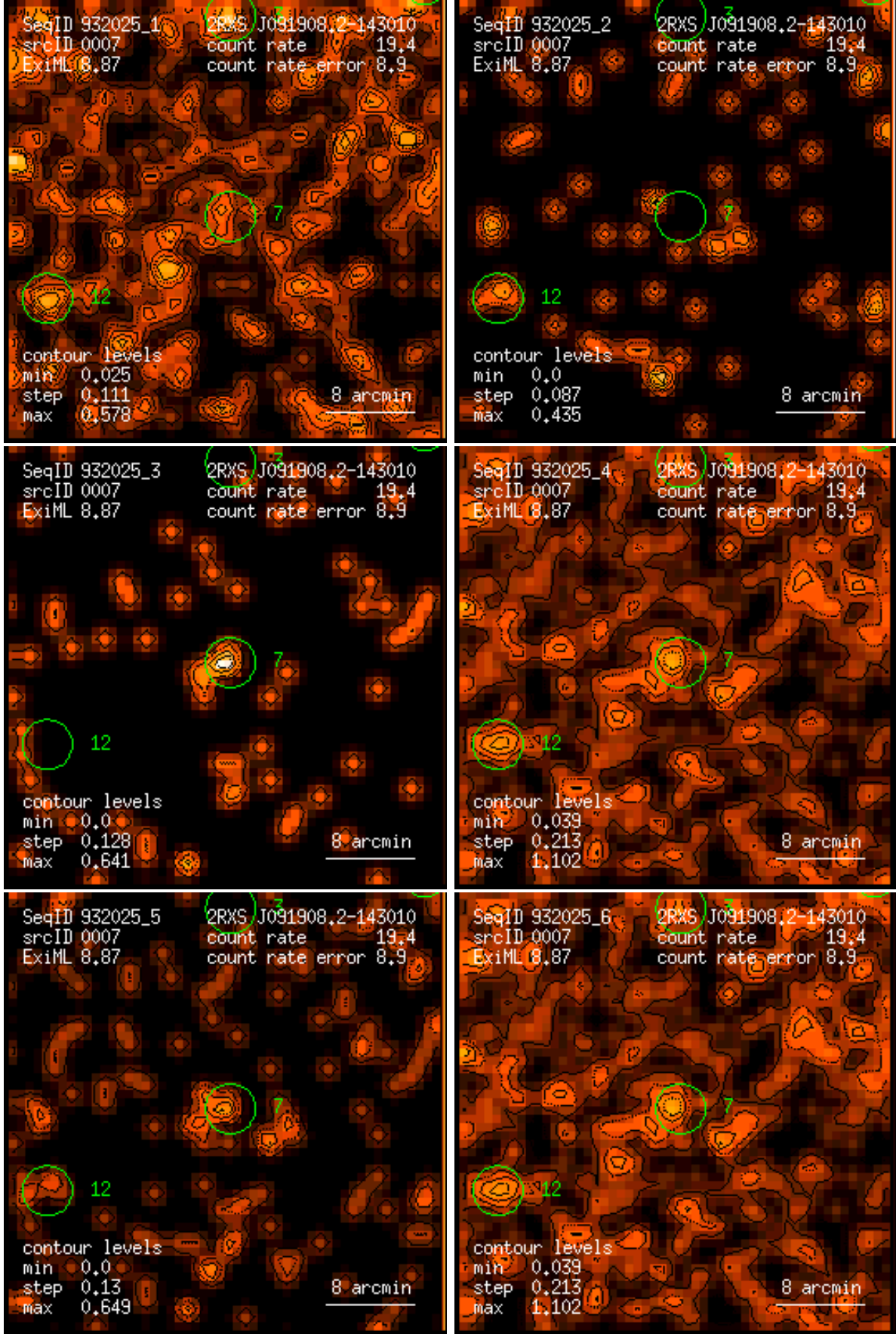
Figure 7: RASS 932025: detection 0007: band rate images, Gaussian filter: (1) PSPC channels 11 – 41, (2) 52 – 90, (3) 91 – 201, (4) 11 – 235, (5) 52 – 201, (6) 11 – 201. Broad band rates in counts/ks. Band rate contour levels in counts/ks/arcmin 2 .
