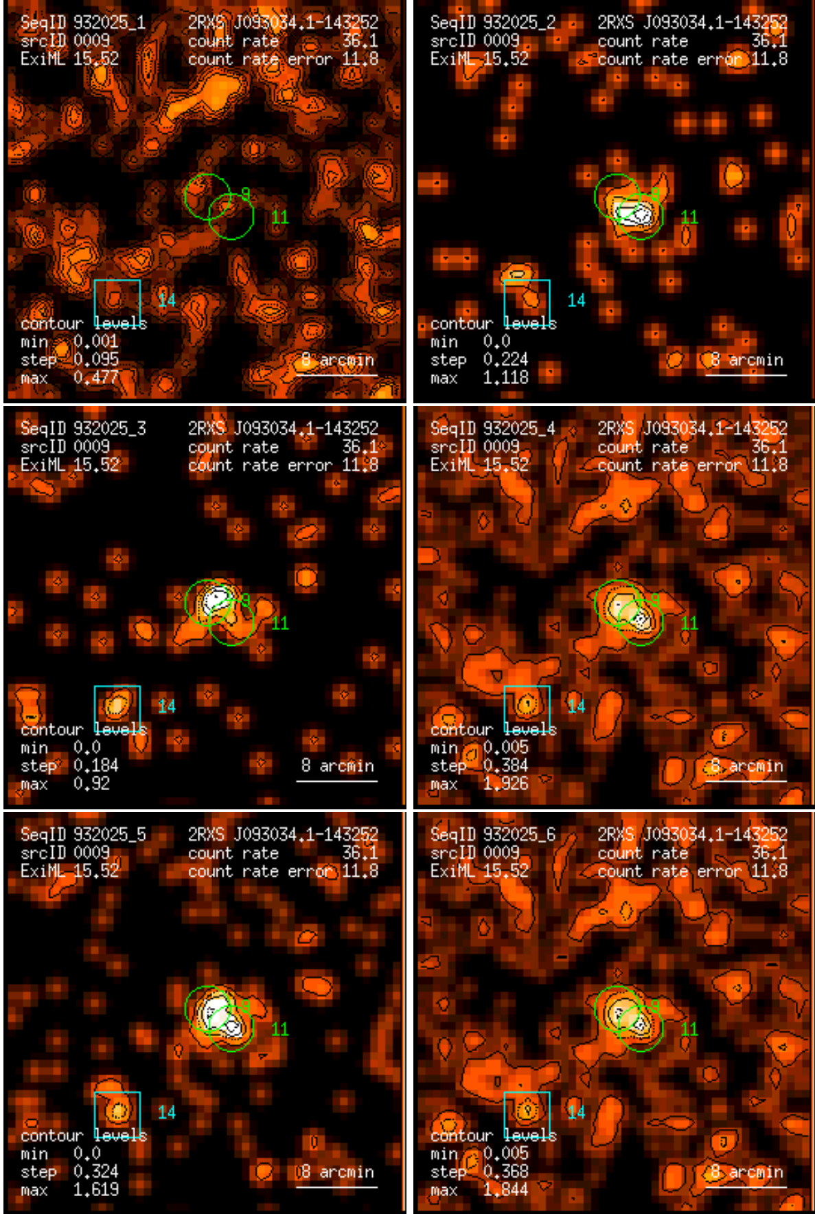
Figure 9: RASS 932025: detection 0009: band rate images, Gaussian filter: (1) PSPC channels 11 – 41, (2) 52 – 90, (3) 91 – 201, (4) 11 – 235, (5) 52 – 201, (6) 11 – 201. Broad band rates in counts/ks. Band rate contour levels in counts/ks/arcmin 2 .
