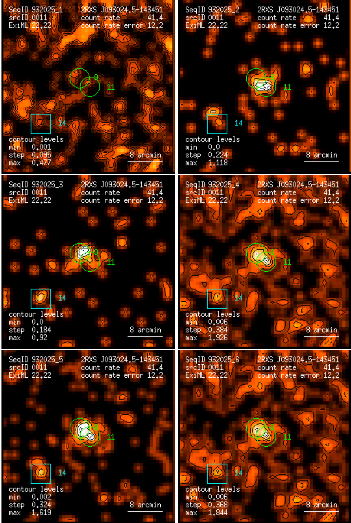
Figure 11: RASS 932025: detection 0011: band rate images, Gaussian filter: (1) PSPC channels 11 – 41, (2) 52 – 90, (3) 91 – 201, (4) 11 – 235, (5) 52 – 201, (6) 11 – 201. Broad band rates in counts/ks. Band rate contour levels in counts/ks/arcmin 2 .
