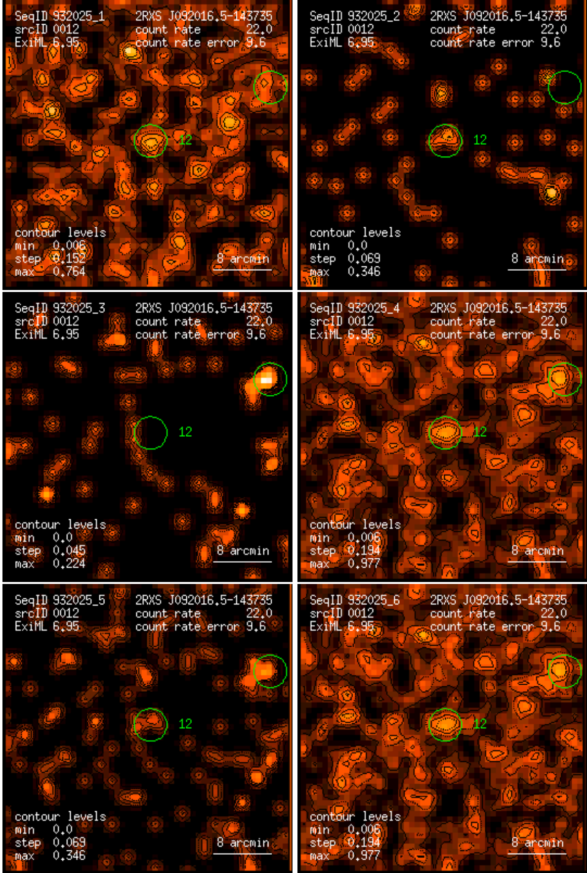
Figure 12: RASS 932025: detection 0012: band rate images, Gaussian filter: (1) PSPC channels 11 – 41, (2) 52 – 90, (3) 91 – 201, (4) 11 – 235, (5) 52 – 201, (6) 11 – 201. Broad band rates in counts/ks. Band rate contour levels in counts/ks/arcmin 2 .
