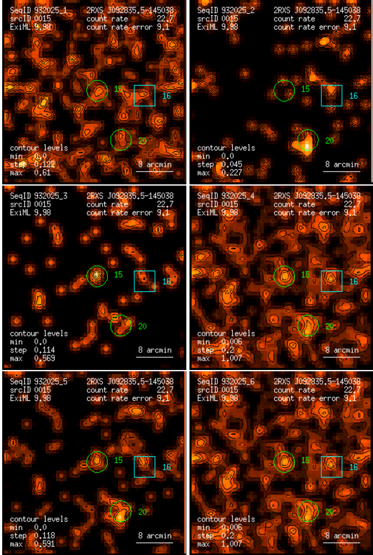
Figure 15: RASS 932025: detection 0015: band rate images, Gaussian filter: (1) PSPC channels 11 – 41, (2) 52 – 90, (3) 91 – 201, (4) 11 – 235, (5) 52 – 201, (6) 11 – 201. Broad band rates in counts/ks. Band rate contour levels in counts/ks/arcmin 2 .
