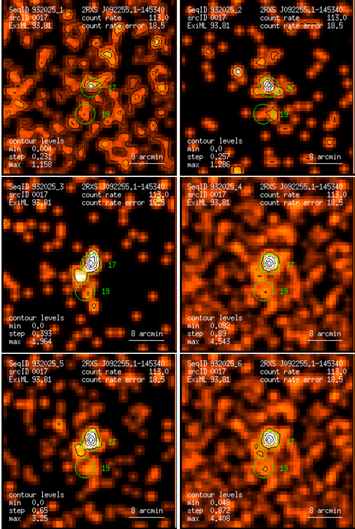
Figure 17: RASS 932025: detection 0017: band rate images, Gaussian filter: (1) PSPC channels 11 – 41, (2) 52 – 90, (3) 91 – 201, (4) 11 – 235, (5) 52 – 201, (6) 11 – 201. Broad band rates in counts/ks. Band rate contour levels in counts/ks/arcmin 2 .
